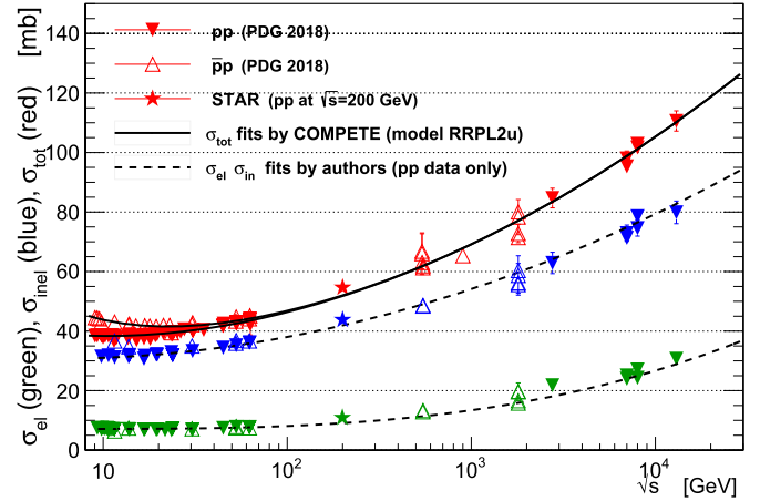
Fig. 7. Comparison of STAR results on \sigma_{tot} , \sigma_{inel} and \sigma_{el} with the world data for data below 1.8 TeV [22], the Tevatron [4–7] and the LHC experiments [1,23–25,27,28]. The COMPETE prediction for \sigma_{tot} is also shown. The dashed curves, represent STAR fits to \sigma_{inel} and \sigma_{el} using the same function as used by COMPETE. STAR data points were not used in the fit.
