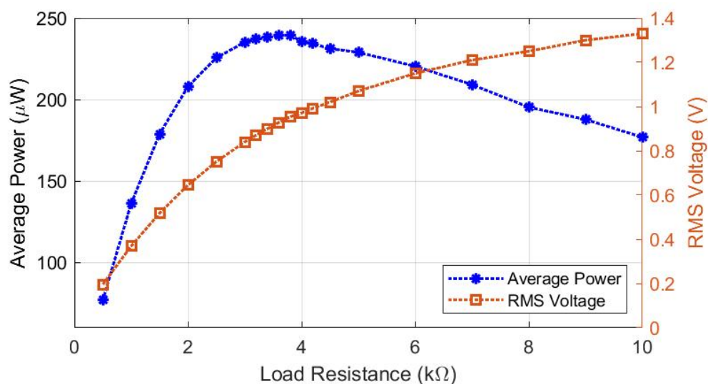
Figure 10. Average power and rms voltage versus resistive load for the EWPT receiver in a 50 \mu T_{rms} magnetic field.
