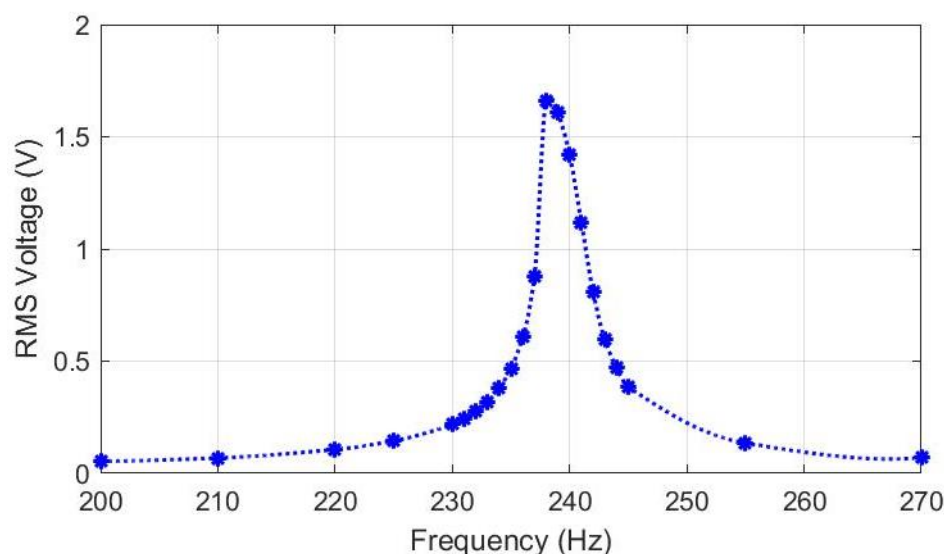
Figure 9. Frequency response of the open circuit EWPT receiver at 50 \mu T_{rms} .
