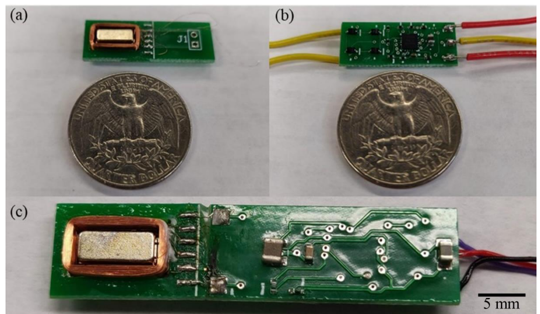
Figure 5. (a) Mounting PCB with micro-receiver compared to a US quarter dollar (USD 0.25). (b) PMC board compared to a US quarter dollar (c) Full micro-receiver and PMC subassembly.
