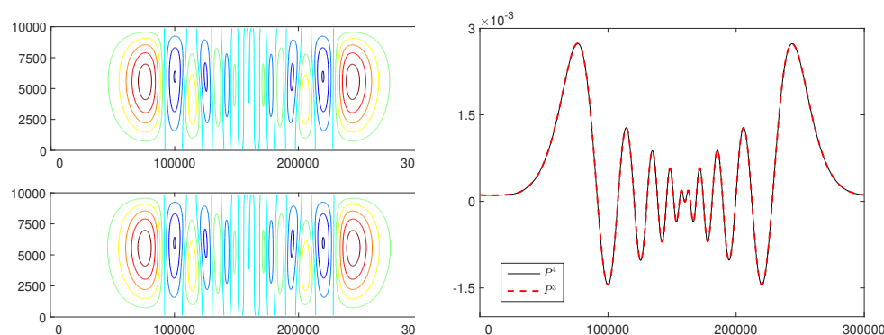
FIG. 8. Example 8: Potential temperature perturbation \Delta\Theta at t = 3000 s. Left: The contours of \Delta\Theta obtained with our fourth-order (top-left) and fifth-order (bottom-left) well-balanced DG schemes on 200 \times 200 cells (10 equally spaced contour lines from -0.0015 to 0.003 ). Right: Profiles of \Delta\Theta along the line y = 5000 m.
