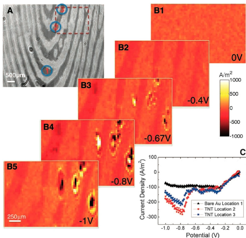
Figure 10. Detection of TNT traces on a fingerprint using the electrochemical current imaging technique. (A) Surface plasmon resonance image of a fingerprint. (B1–B5) Five snapshots recorded while sweeping the potential negatively from 0 to -1.0 V at a rate of 0.05 V/s. The appearance of the “spots” is due to the reduction of TNT particulates. (C) Local voltammograms of the regions with (blue and red dots) and without (black dots) TNT particulates. The electrolyte is 0.5 M KCl. Reprinted with permission from ref 23. Copyright 2010 American Association for the Advancement of Science.
