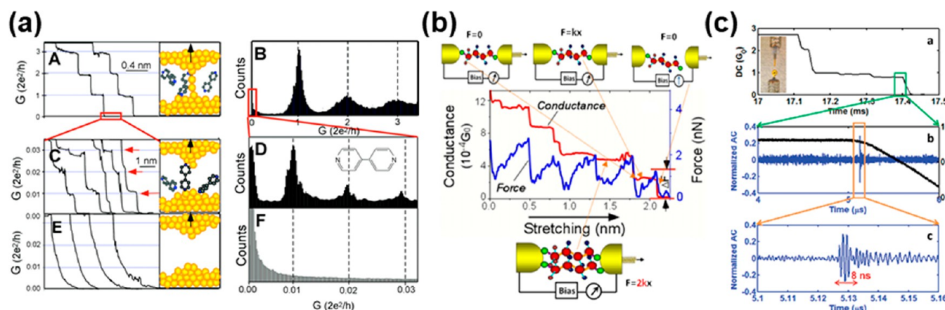
Figure 6. Scanning tunneling microscopy-break junction (STM-BJ) method. (a) STM-BJ using 4,4'-bipyridine molecules. Reprinted with permission from ref 293. Copyright 2018 American American Chemical Society. (b) Conductive atomic force microscopy measurement of Au-thiol binding in Au-octanedithiol-Au molecule junction. Reprinted from ref 38. Copyright 2006 American Chemical Society. (c) AC-modulation of molecular junctions. Reprinted from ref 12. Copyright 2011 American Chemical Society.
