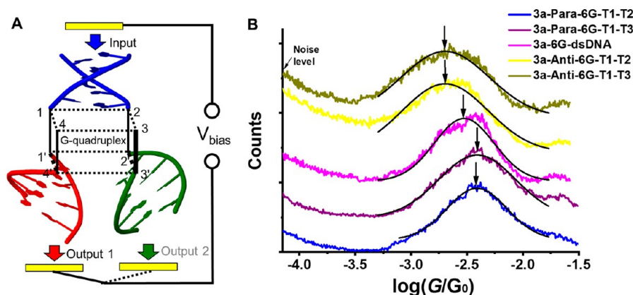
Figure 8. Design and testing of a G-quadruplex-based current splitter. (A) Schematic of the current-splitting element placed between two electrodes. The G4 element (black) plus three DNA duplexes are held between an Au tip and an Au substrate in a break-junction configuration. (B) Conductance histograms of the quadruplex 3 with six layers of guanines. The different conductance histograms represent whether the strands are arranged in an antiparallel or parallel configuration and which of the three duplex terminals (T1, T2, T3) have thiols to bind to the electrodes. The conductance values ( x -axis) are similar for all the DNA structures. For clarity, each histogram was shifted vertically to avoid overlap. Reprinted with permission from ref 232. Copyright 2018 Springer Nature.
