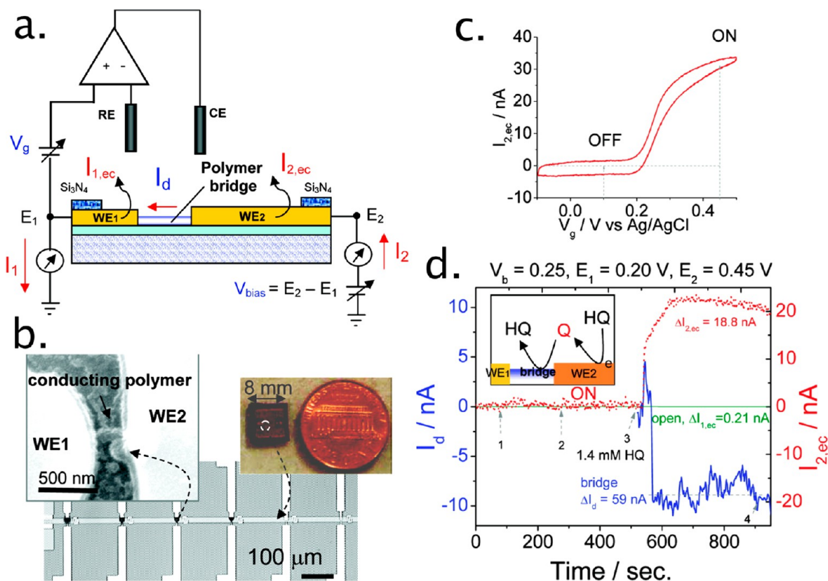
Figure 5. (a) Schematic illustration of a hybrid amperometric and conductometric sensor. WE1 and WE2 represent two working electrodes (source and drain electrodes) connected with a conducting polymer bridge. RE and CE are reference and counter electrodes, respectively. The electrochemical gate potential ( V_g ) E_1 is applied between the drain electrode (WE 1 ) and RE, and a bias voltage ( V_{bias} ) is applied between WE 1 and WE 2 . (b) Optical and scanning electron microscope images of the device made of an array of polymer bridges on a silicon chip. (c) Cyclic voltammogram of 3.9 mM hydroquinone (HQ) on polyaniline-modified microelectrode at 60 mV/s. (d) \Delta I_d and \Delta I_{2,ec} simultaneously recorded during the injections of supporting electrolyte (1–2) and 1.4 mM HQ (3) to a close (bridge) and open polymer bridge (open) amperometric and conductometric device. V_{bias} is 0.25 V, and E_2 is 0.45 V. Inset of (d) illustrates the reaction mechanism in a close polymer bridge device. Reprinted from ref 34. Copyright 2007 American Chemical Society.
