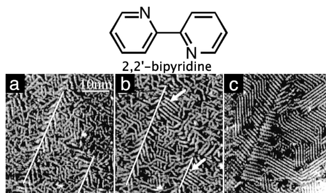
Figure 3. Potential-induced disorder–order transition in a 2,2'-bipyridine monolayer on reconstructed Au(111). Images (a–c) were obtained at sample potentials of 0.11, 0.24, and 0.38 V versus SCE, respectively, in aqueous 0.10 M NaClO 4 . Lines in (a) and (b) indicate the direction of the reconstruction strips. Arrows in (b) point to the formation of the ordered phase as the potential is raised to 0.24 V. Reprinted from ref 94. Copyright 1996 American Chemical Society.
