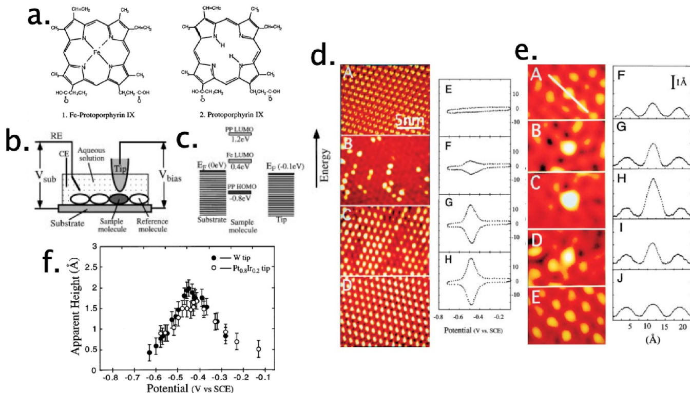
Figure 2. (a) Iron protoporphyrin (FePP, left) and protoporphyrin (PP, right) molecules. (b) Schematic diagram of a scanning tunneling microscope (STM) with control of the electrochemical potential of the tip and surface for investigations of single-molecular electron transfer. (c) Energy level diagrams of Fe(III)-protoporphyrin IX and protoporphyrin IX and their relation to the Fermi levels of the substrate and tip. (d) STM images of FePP/PP mixed monolayers on graphite containing FePP and PP at the ratio of (A) 0:1, (B) 1:4, (C) 4:1, and (D) 1:0 and (E–H) are the corresponding cyclic voltammograms. (e) STM image of FePP molecule embedded in an ordered matrix of PP molecules when the substrate was held at (A) -0.15 , (B) -0.30 , (C) -0.42 , (D) -0.55 , and (E) -0.65 V versus SCE reference electrode. (f) Apparent height of FePP relative to PP as a function of the substrate potential via Pt–Ir tip and W tip. Figures (a–d) reprinted with permission from ref 87. Copyright 1996 American Physical Society.
