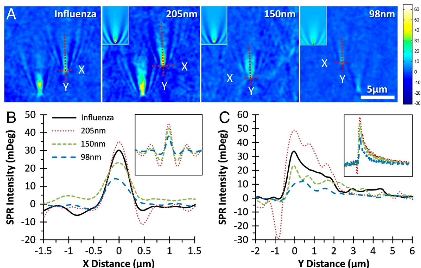
Figure 11. (A) Surface plasmon resonance microscopy (SPRM) images of H1N1 influenza A virus and three different-sized silica nanoparticles in phosphate-buffered saline (PBS) buffer. (Insets) Nanoparticle images generated by numerical simulation. (B and C) The SPR intensity profiles of selected particles along X and Y directions (indicated by dashed lines in A, respectively). (Insets) Corresponding profiles from simulated images. Reprinted with permission from ref 28. Copyright 2010 National Academy of Sciences.
