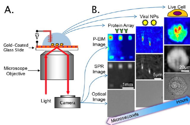
Figure 9. Principles and applications of plasmonic-based electrochemical impedance microscopy (P-EIM) microscopy. (A) Schematic of P-EIM imaging principle: Surface plasmon waves are created optically with a laser or light-emitting diode beam incident on the metal film via a prism or high-numerical-aperture objective at a resonant angle, and the reflected beam creates a surface plasmon resonance microscopy (SPRM) image. The resonant angle is sensitive to changes in refractive index near the metal surface, which is widely used to study molecular binding processes. In addition, the resonant angle is also sensitive to surface charge density, which produces the electrochemical impedance image when an ac voltage is applied to the surface. (B) Optical, SPRM, and P-EIM images of a protein microarray, viral nanoparticles (NPs) and a mammalian cell.
