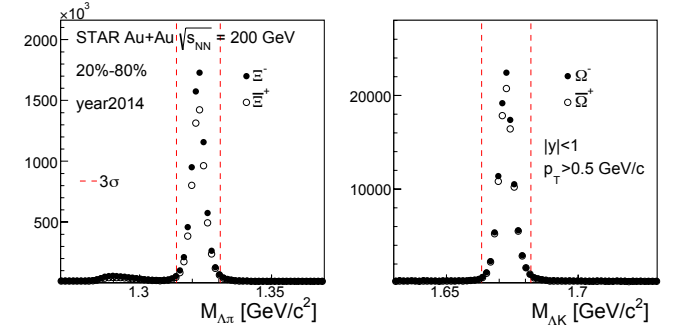
FIG. 1. (Color online) Invariant mass distributions of \Xi^- ( \Xi^+ ) and \Omega^- ( \Omega^+ ) for 20%-80% centrality in Au+Au collisions at \sqrt{s_{NN}} = 200 GeV taken in 2014. Vertical dashed lines indicate three standard deviations ( 3\sigma ) from the peak positions, assuming a normal distribution.
