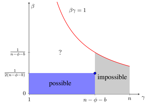
Fig. 1: Achievability of (\beta, \gamma) for complete graphs
