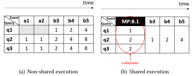
Figure 2: Intermediate aggregate count storage for stream I = (a1, a2, b3, b4, b5) under: (a) non-shared execution of plan P1; (b) execution sharing sub-pattern B^+ for queries q1 , q2 , and q3 as per plan P2 from Figure 1.
