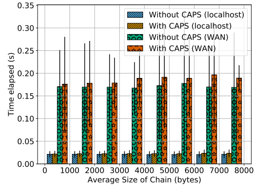
Figure 13: Handshake latency versus the average certificate chain size sent by the domain. Error bars represent standard error.
