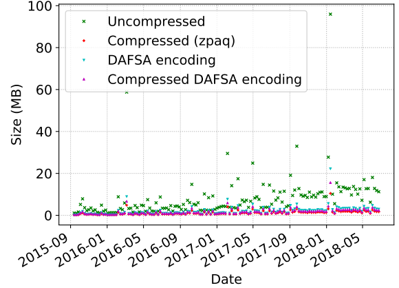
Figure 6: Size of update set (added name set and deleted name set) in different formats over time.
