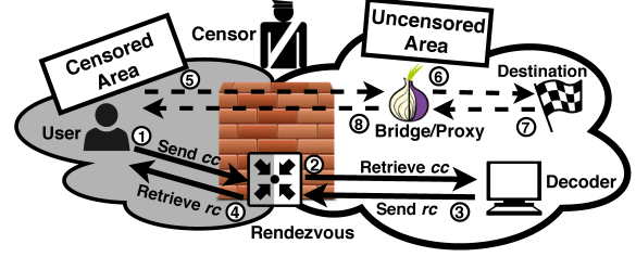
Fig. 1. Censorship circumvention bootstrapping problem. Censored user sends a coverttext to the decoder, who replies with another coverttext including proxy’s details. Then, the censored user can access censored information through the proxy. We focus on the bootstrapping process (solid arrows).
