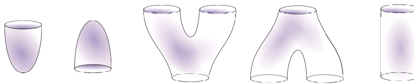
Figure 9. The building blocks of a surface. Given a scalar function f defined on a surface M , Theorem 2 asserts that we can decompose the surface into the building block pieces appear in above. These pieces are genus zero surfaces with a single boundary component (disk), genus zero surfaces with three boundary components (pair of pants), and a genus zero surface with two boundary components (cylinder).
