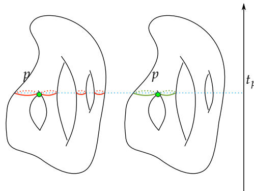
Figure 4. For t_p a critical value, on the left, the set f^{-1}(t_p) consists of a singular set C_p and two of simple closed curves. On the right, only the critical set C_p is shown, which is the connected component of f^{-1}(t_p) that contains the critical point p .
