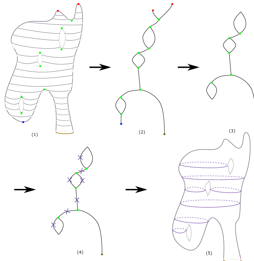
Figure 22. A Reeb graph can be used to segment a surface into a collection of topologically consistent patches. (1) The surface M , with a scalar function f , is given as an input. (2) The Reeb graph of R(M, f) is calculated. (3) The deformation retract graph R'(M, f) of the graph R(M, f) is calculated. (4) For each edge in the graph R'(M, f) , we select a point. (5) We select the curves on the manifold M that corresponds to the points that were selected in the previous step.
