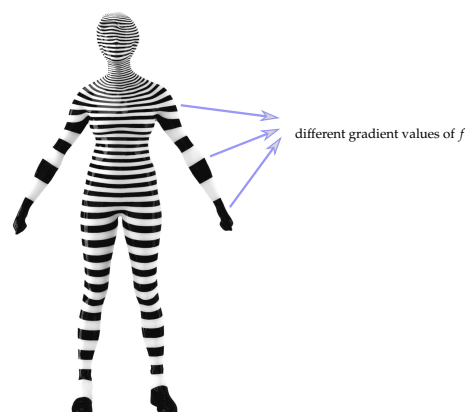
Figure 14. The arm of the female character mesh corresponds to a single arc in the Reeb graph associated with the scalar function indicated on the mesh. Observe that the gradient of this scalar function varies along this arm, which makes it hard to parametrize the mapping between the Reeb graph and the corresponding regions on the mesh.
