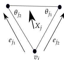
Figure 16. Computing the divergence at vertex v_i .
