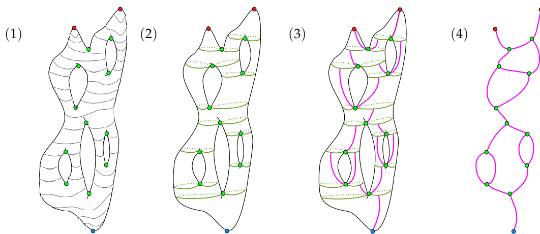
Figure 6. Summary of the sequential algorithm. (1) The input of the algorithm is a manifold M with a scalar function f . (2) Computing the critical sets. (3) For each saddle point or minimum, we compute the ascending paths (4) creating the edges of the Reeb graph by the information encoded in the start vertex of the ascending vertex and its termination critical set.
