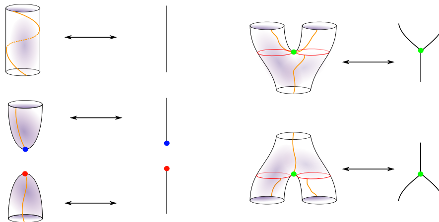
Figure 10. The restriction of the Reeb graph on the building blocks of a surface along with the part of the ascending paths in that part of the surface. Around each critical point, the structure of the ascending curves (orange) is identical to the structure of the Reeb graph. More precisely, the quotient space of the restriction of the function on the ascending curves the critical sets around a critical point (these are the curves highlighted by orange and red in the figure) is identical to the quotient space of the manifold locally.
