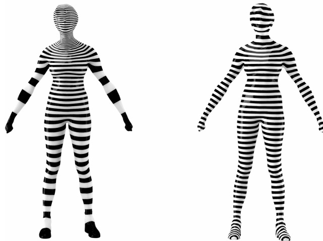
Figure 17. Obtaining a unit gradient scalar field.
