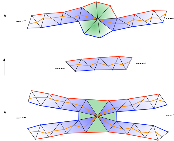
Figure 7. The set of vertices, edges, and faces in the mesh M , which f^{-1}(t) intersects. The top two figures depict cases where t is a regular value. The top figure shows an example of when there exists a vertex v in M , such that v \in f^{-1}(t) . The second figure shows the case where no such a vertex exists. In other words, f^{-1}(t) intersects only edges and faces of M . The third figure is an example of the local neighborhood, a critical point of f or when f^{-1}(t) contains a critical point. The purple simplices represent the set CR_f(t) . The union of the green and purple simplices represents the set CR_f(t) . The blue edges and nodes are the edges in the complexes that are shown in the figure and nodes in \overline{CR_f(t)} , which have f -values less than or equal to t . The red edges and nodes are the edges in the complexes shown in the figure and nodes in \overline{CR_f(t)} , which have f -values that are higher than or equal to t .
