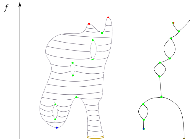
Figure 2. An example of a Reeb graph (right) of a scalar function (left) defined on a surface with a boundary.
