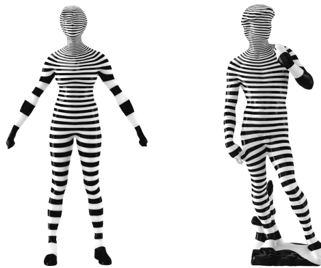
Figure 25. Example of Poisson fields on Triangulated meshes. In both characters, a single vertex, which is the highest node in the head of the character, was chosen to be the constrained vertex required to solve the Poisson equation. Observe how this scalar function follows the geometry of the mesh.
