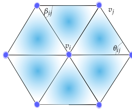
Figure 24. The angles \theta_{ij} and \beta_{ij} are defined with respect to an edge [v_i, v_j] .
