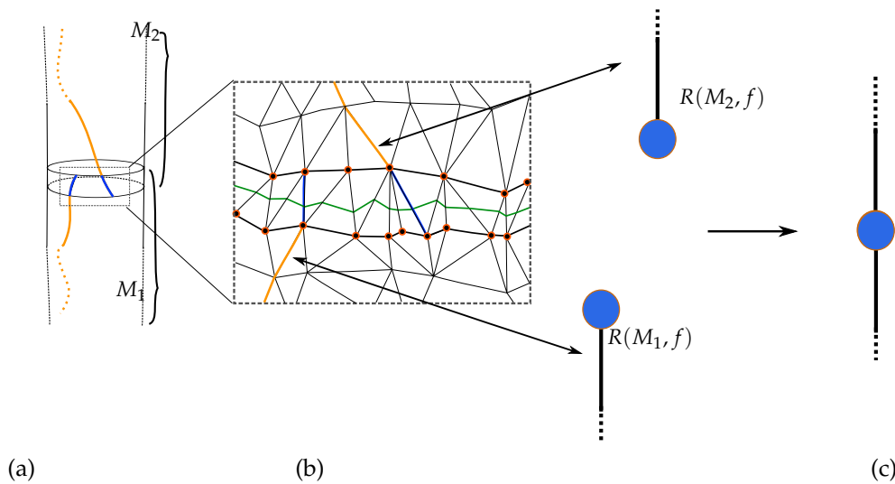
Figure 12. An illustration of the gluing stage. (a) At this stage, two ascending paths from all submanifolds have been calculated. In the case when two consecutive submanifolds share a crossing edge, such as the case in the illustrative figure, the ascending path of the lower submanifold M_1 gets terminated at the at a crossing edge. Similarly, an ascending path from the higher submanifold M_2 gets initiated at a crossing edge. (b) A zoomed version of Figure (a) shows the two crossing edges that determine uniquely two nodes in the Reeb graphs R(M_1, f) and R(M_2, f) . The fact that these two edges belong to the same connected component in the inverse image of the regular crossing value is used to glue the graphs R(M_1, f) and R(M_2, f) along the blue nodes to obtain the graph in Figure (c).
