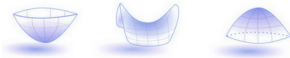
Figure 1. Minimum, Saddle, and Maximum, respectively.
