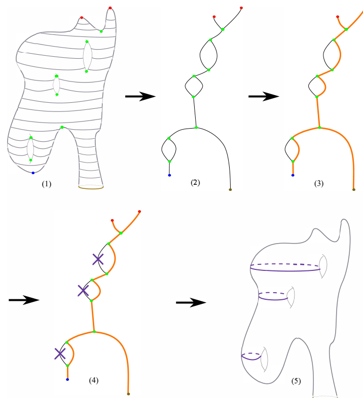
Figure 20. The steps of the cutting system algorithm. (1) mesh M with a scalar function defined on it are given. (2) The Reeb graph R(M, f) is computed. (3) We compute a spanning tree of R(M, f) . (4) We select all edges in the graph that do not belong the spanning tree we computed in (3) and then we select an interior point on each one of these edges. (5) For each interior point, we used our augmented Reeb graph algorithm to compute the circle that corresponds to it on the mesh.
