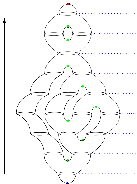
Figure 8. Given a Morse function f on a surface M , we can slice M , so that, around each critical value t , the submanifold M_{[t-\epsilon, t+\epsilon]} is a disjoint union of simple building blocks: pair of pants, topological cylinders, and topological disks.
