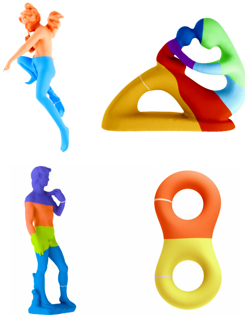
Figure 23. Examples of segmentation of higher genus surfaces into a pair of pants using our Reeb graph algorithm.
