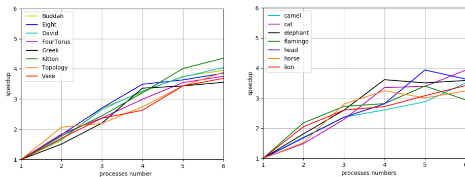
Figure 18. Speedups obtained by our parallel Reeb graph algorithm.
