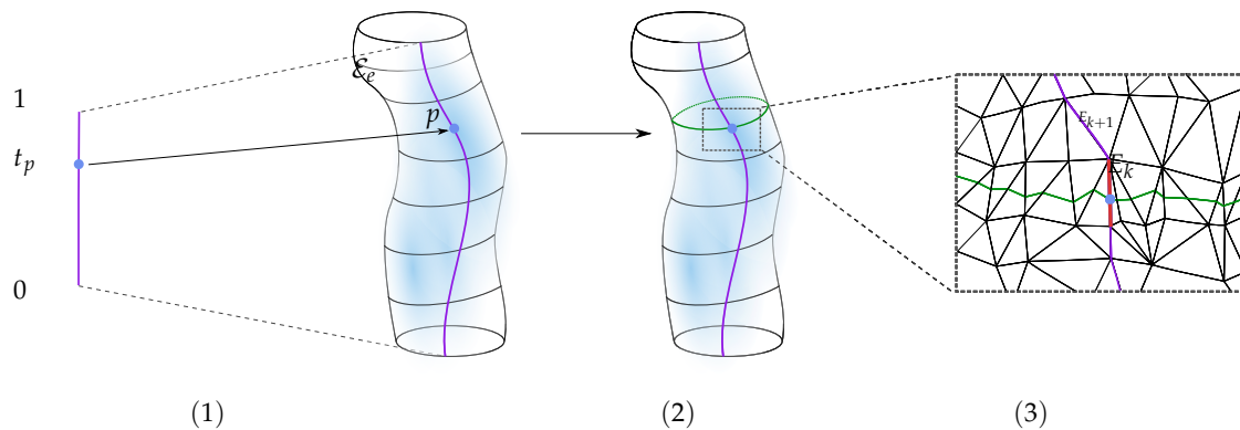
Figure 13. An illustration of the data retrieval procedure. (1) A value t_p is selected from the interval (0, 1) . (2) This value is used to determine a point p on the Reeb graph edge \mathcal{E}_e . (3) This point is contained in an edge E_k on the mesh M . This edge is used to determine the circle Cr_p
