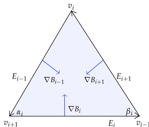
Figure 15. The gradients of hat functions of a triangle.
