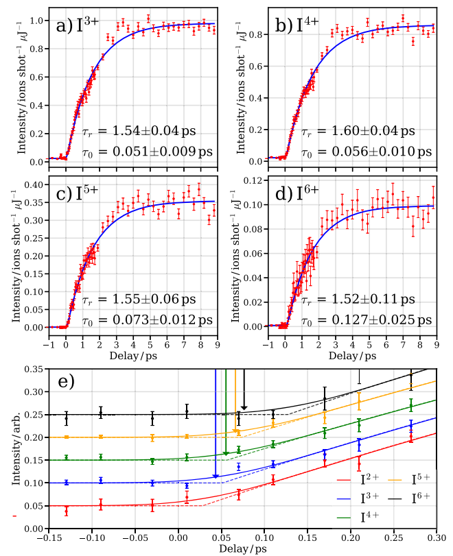
Figure 7. Time-resolved yields of the low KE ( \sim 0.2 – 0.4 eV) ions for (a) I^{3+} , (b) I^{4+} , (c) I^{5+} and (d) I^{6+} . Experimental data with statistical error bars are shown in red, while fits using the function shown in the text are plotted in blue. The exponential rise time, \tau_r , and time offset, \tau_0 , for each fit are overlaid. Panel (e) displays time-resolved yields of low KE I^{2+} to I^{6+} ions shortly after time-zero. Fits for each ion are plotted both with (solid lines) and without (dashed lines) Gaussian convolution by the instrument response function. Offset times predicted by the over-the-barrier model, relative to the fitted offset time for I^{2+} are displayed for each ion as colored arrows.
