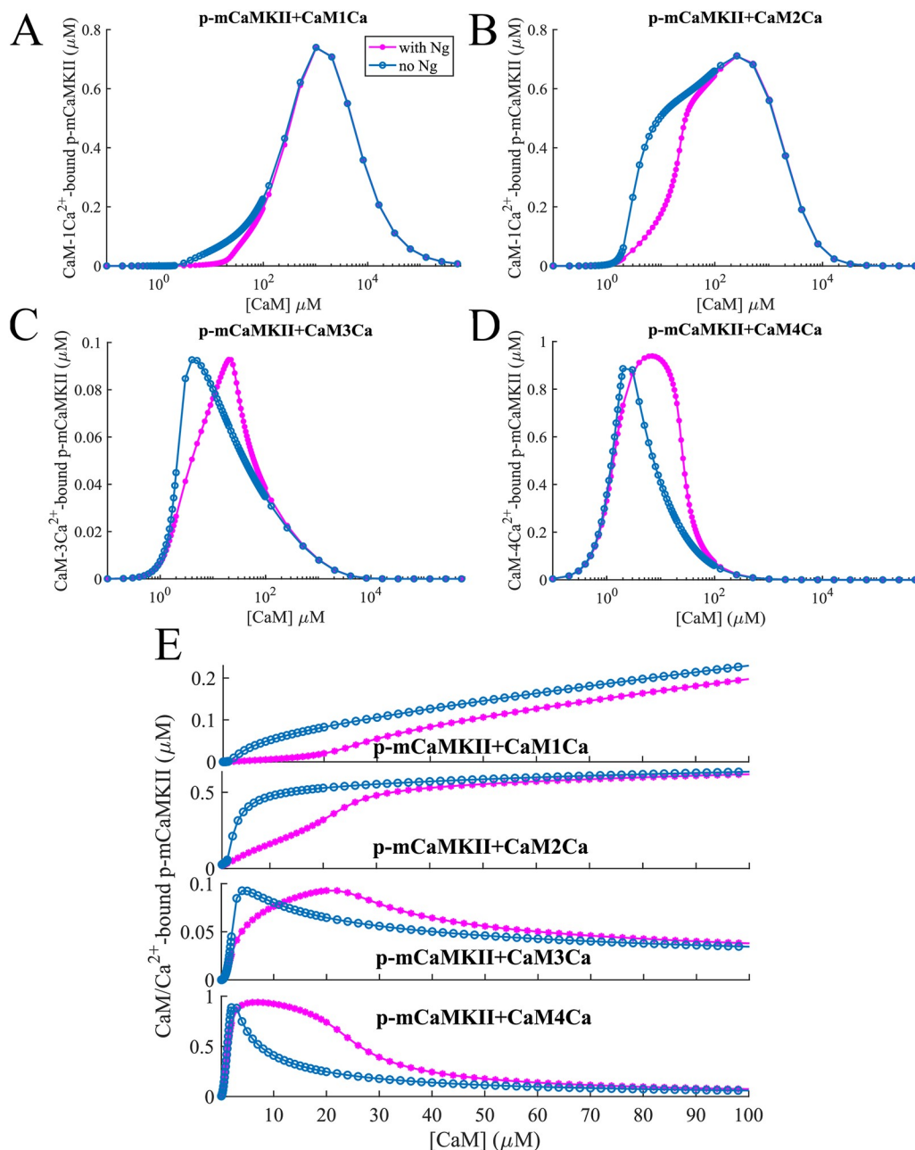
Fig 3. mCaMKII phosphorylation. Dose response of phosphorylated mCaMKII molecules bound to (A) 1-, (B) 2-, (C) 3- and (D) 4-calcium states of CaM- \text{Ca}^{2+} as shown in Fig 2. At low [CaM], the “multi-calcium-bound” forms of calmodulin play an important role. This is amplified by the fact that these forms when bound to CaMKII give it higher phosphorylation rates (Table 1). (E) shows the same effect for physiologically relevant [CaM]. In these simulations, input [\text{Ca}^{2+}] = 10 \mu\text{M} constant.
