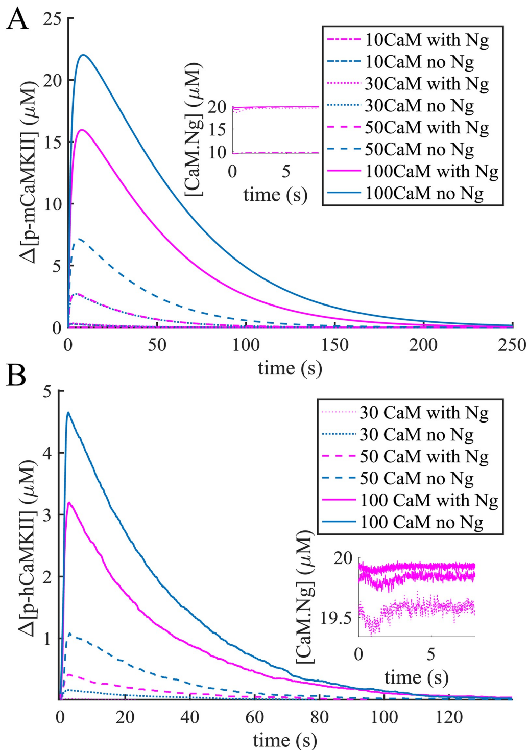
Fig 6. CaMKII phosphorylation in response to a calcium spike. The rise in CaMKII phosphorylation level as a response to a [\text{Ca}^{2+}]_{\text{free}} = 10 \mu\text{M} spike with monomers (A) and holoenzymes (B) for different conditions. The response of the holoenzyme at [\text{CaM}] = 10 \mu\text{M} was not significant and is not shown here. The insets show that when [\text{CaM}] > 20 \mu\text{M} , nearly 20 \mu\text{M} of it is bound to Ng.
