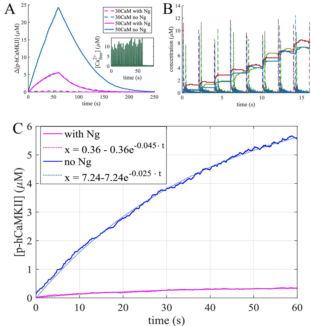
Fig 9. Responses to trains of 30 Ca^{2+} pulses. (A) An average phosphorylation of CaMKII holoenzyme in response to 30 Ca^{2+} pulses at 0.5 Hz averaged over 30 simulations with 63 holoenzymes and 30 \mu\text{M} , and 50 \mu\text{M} calmodulin. (B) Three individual simulations: the response of hCaMKII phosphorylation level (solid lines) change to the calcium spikes (dashed lines). (C) Fitting the leaky integrator. The average response to 30 Ca^{2+} pulses was fitted to a curve of the form x = k - k \cdot e^{-a \cdot t} with and without Ng and [CaM] = 30 \mu\text{M} , with the curve fitting tool from MATLAB. The parameters obtained are: k = 7.24 , a = 0.025 with an R^2 = 0.9979 without Ng and k = 0.36 , a = 0.045 with an R^2 = 0.9683 with Ng. Thus Ng not only changes the leaking rate of the integrator, but significantly lowers the maximum possible phosphorylation level.
