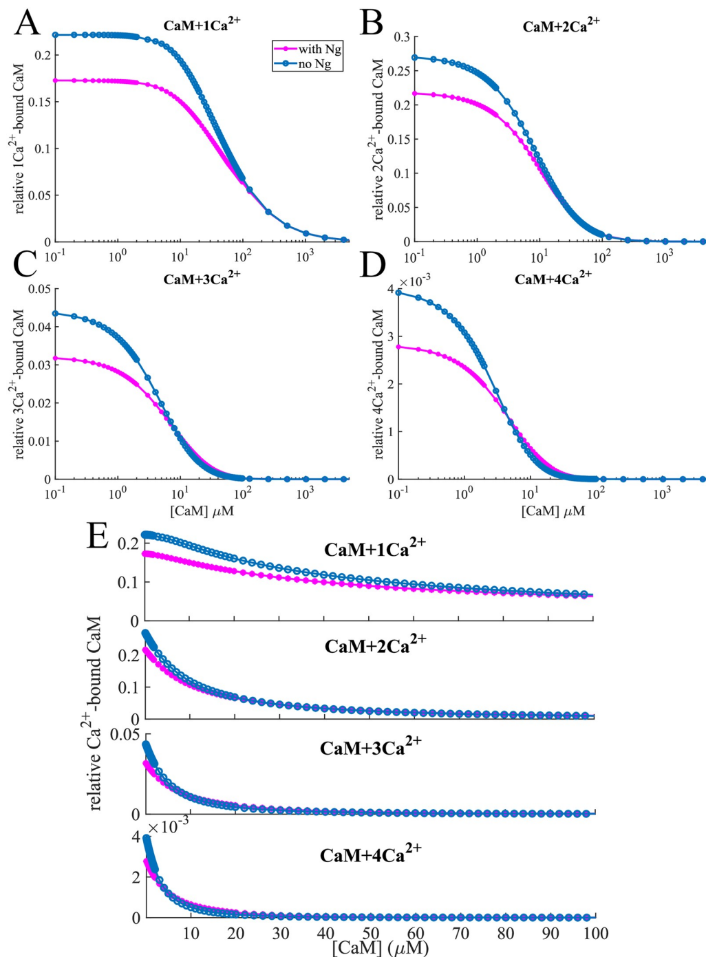
Fig 2. CaM binding calcium. Relative concentration of (A) 1-, (B) 2-, (C) 3- and (D) 4-calcium-bound calmodulin vs. total [CaM] at constant [Ca 2+ ] = 10 μM. For most of the calcium-bound forms, the relative concentration is lower in the presence of neurogranin. However, in the case of 3- and 4-calcium-bound calmodulin the situation is reversed for certain [CaM]: Ng competes with Ca 2+ for free calmodulin, which allows a regime where the concentration of these “multi-calcium-bound” forms is higher. As the concentration of calmodulin is further increased, the [Ca 2+ ]:[CaM] ratio decreases and these forms die out. Thus at high [CaM] the effects of Ng are diminished. (E) shows the same effect for physiologically relevant [CaM].
