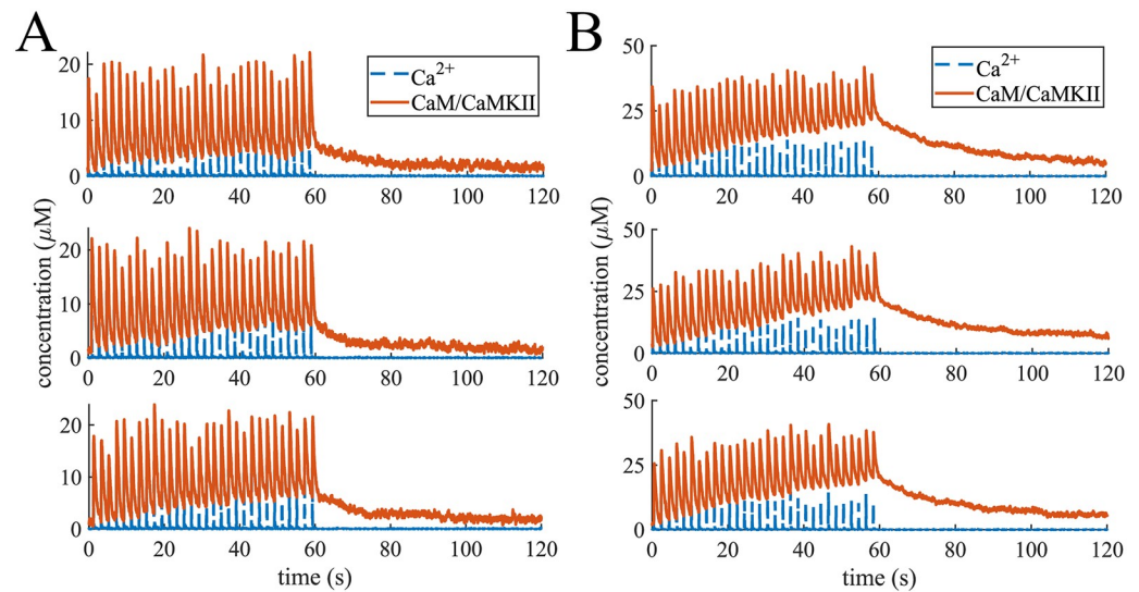
Fig 10. Responses to trains of 30 \text{Ca}^{2+} pulses. 3 representative curves of CaMKII subunits in the holoenzyme binding CaM in response to \text{Ca}^{2+} spikes at [\text{CaM}] = 50 \mu\text{M} with (A) and without (B) Ng.
