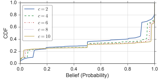
Fig. B.1: The effect of the parameter c on the distribution of beliefs for all nodes in the LAX campaign.
