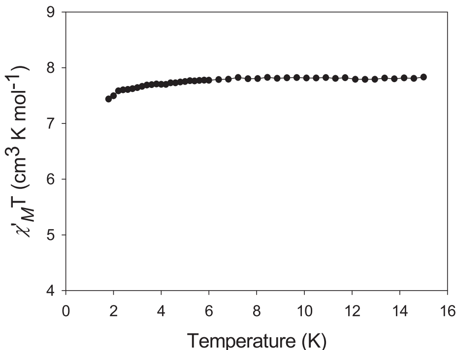
Fig. 5. In-phase ( \chi'_m , as \chi'_m T ) vs T ac susceptibility for vacuum-dried 1 \cdot \frac{3}{2} \text{H}_2\text{O} at 1000 Hz. The solid line is a guide for the eye.
