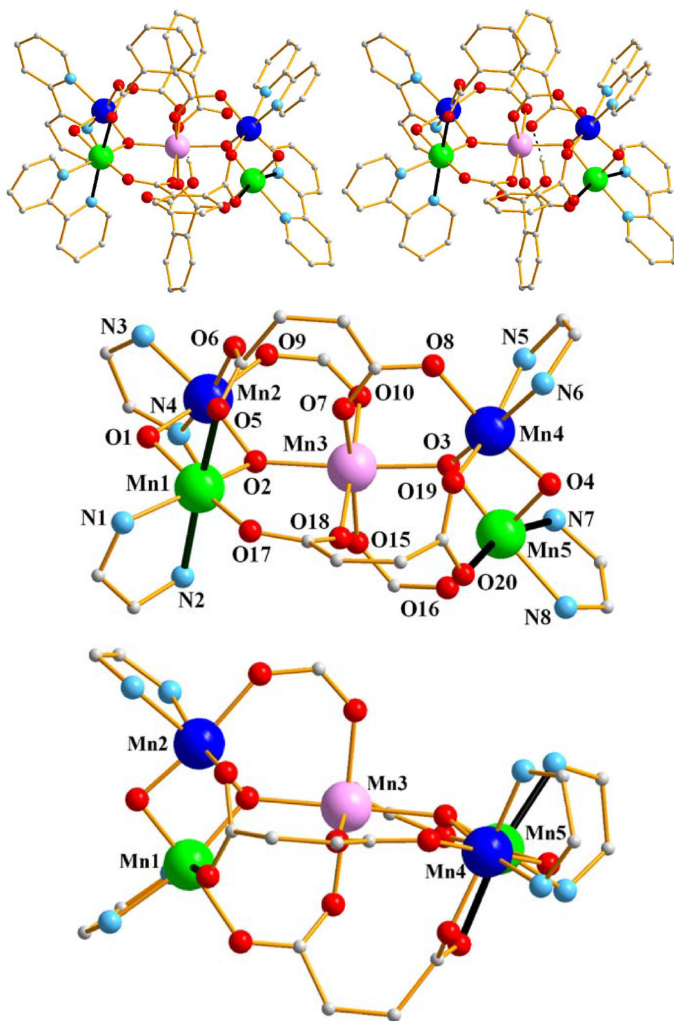
Fig. 1. (top) a stereopair of the complete cation of 1, with the intra-cation O14-H14...O11 hydrogen-bond indicated by the dashed line; (middle) a labeled simplified representation; and (bottom) its core from a viewpoint that emphasizes the near-perpendicular arrangement of the two Mn II Mn III Mn IV triangles fused at the central Mn II (Mn3). H atoms have been omitted for clarity. Thicker bonds in black denote Jahn-Teller elongation axes. Color code: Mn IV blue; Mn III green; Mn II violet; O red; N sky blue; C grey. ((Color online.))
