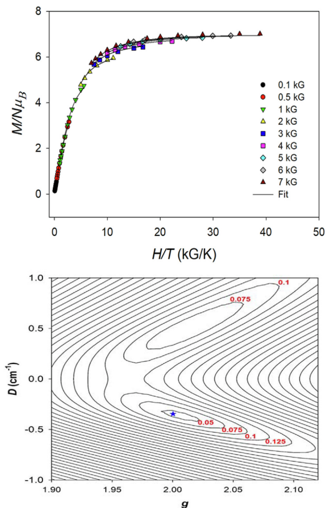
Fig. 4. (top) plot of reduced magnetization ( M/N\mu_B ) vs. H/T data for 1\cdot^{3/2}\text{H}_2\text{O} at the indicated applied dc fields. The solid lines are the fit of the data; see the text for the fit parameters. (bottom) root-mean-square g vs D error surface as a 2-D contour plot for the fit of M/N\mu_B vs H/T for 1\cdot^{3/2}\text{H}_2\text{O} . The asterisk indicates the best-fit minimum corresponding to the fit parameters in the text. ((Color online.))
