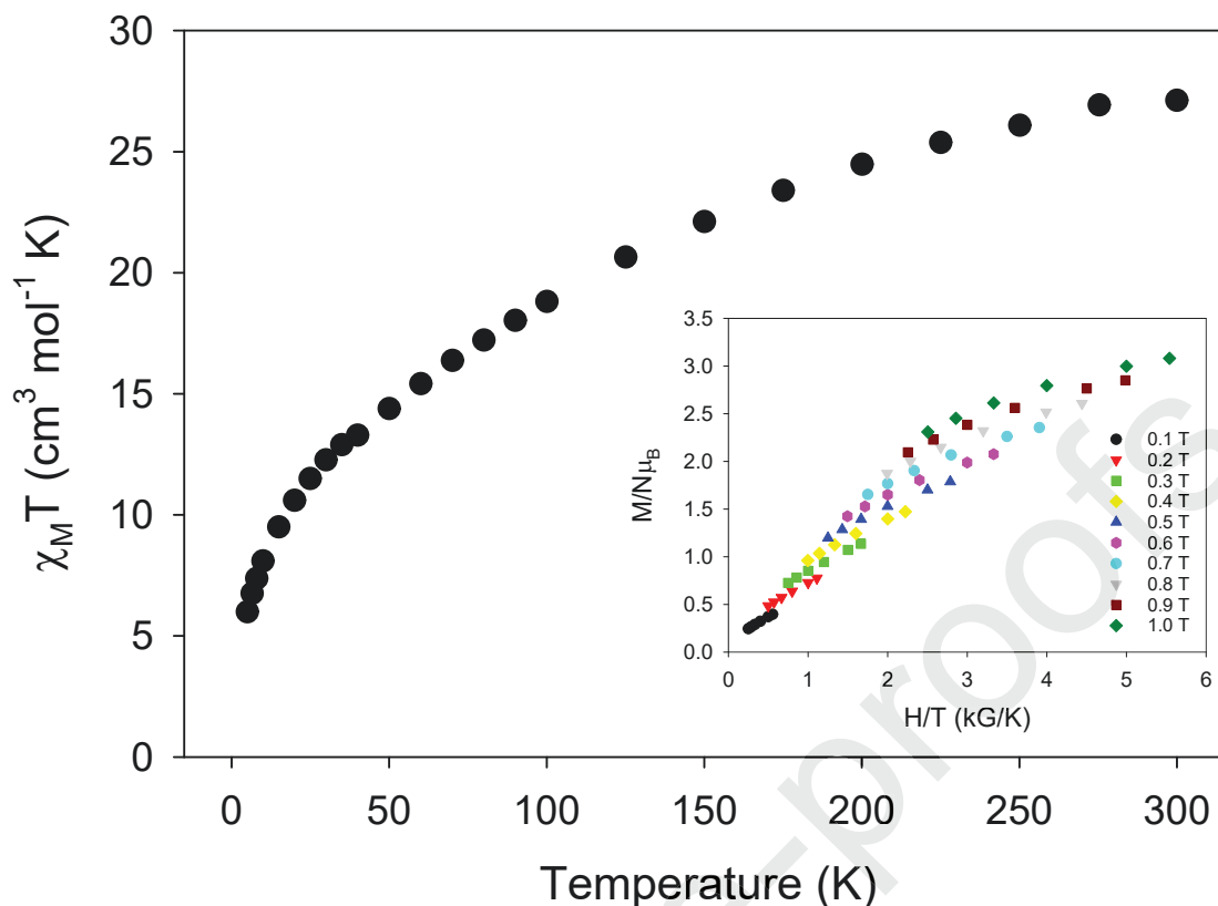
Fig. 7. Plot of \chi_M T vs. T for 1 \cdot 3\text{H}_2\text{O} in a 1 kG field. (inset) Reduced magnetization plot of M/N\mu_B vs. H/T for 1 \cdot 3\text{H}_2\text{O} at the indicated applied fields.
