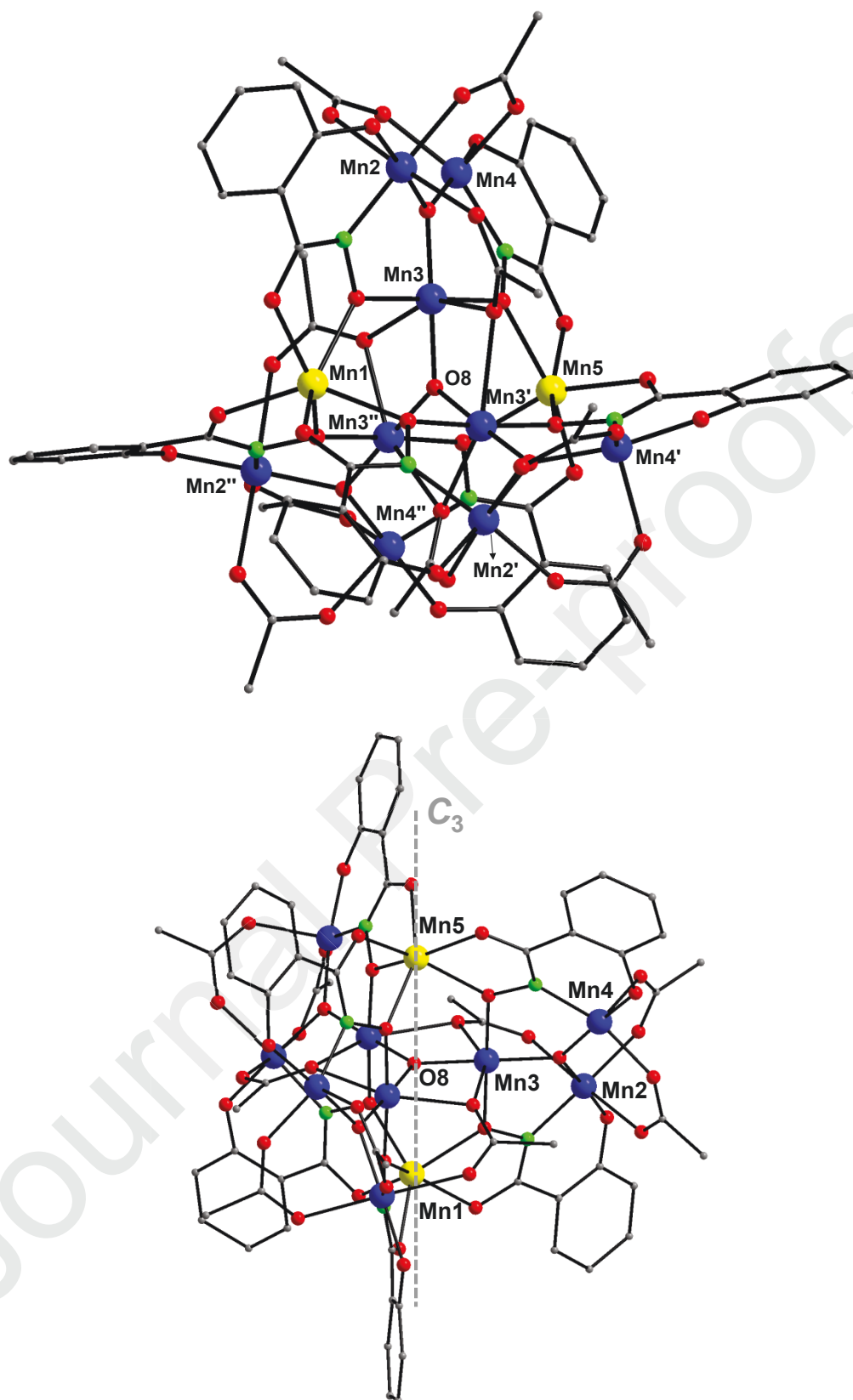
Fig. 1. Partially labeled representation of the anion of complex 1 (top), and a different view of its structure along the C_3 -axis (bottom). H atoms are omitted for clarity. Color
