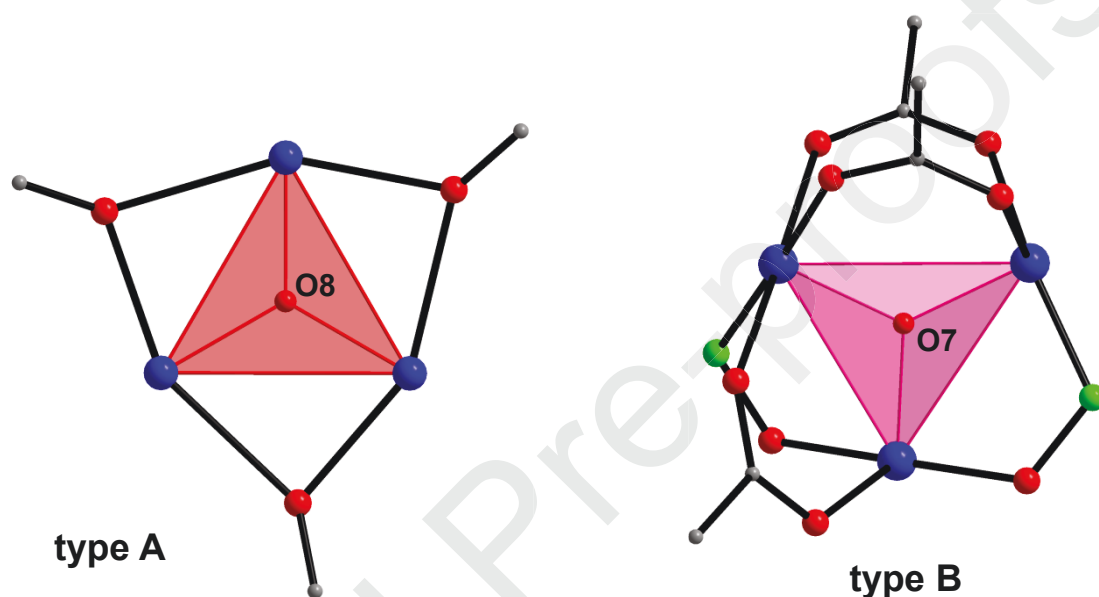
Fig. 2. Representation of the two types of triangular subunits present in the structure of complex 1 . Color scheme as in Fig. 1.
