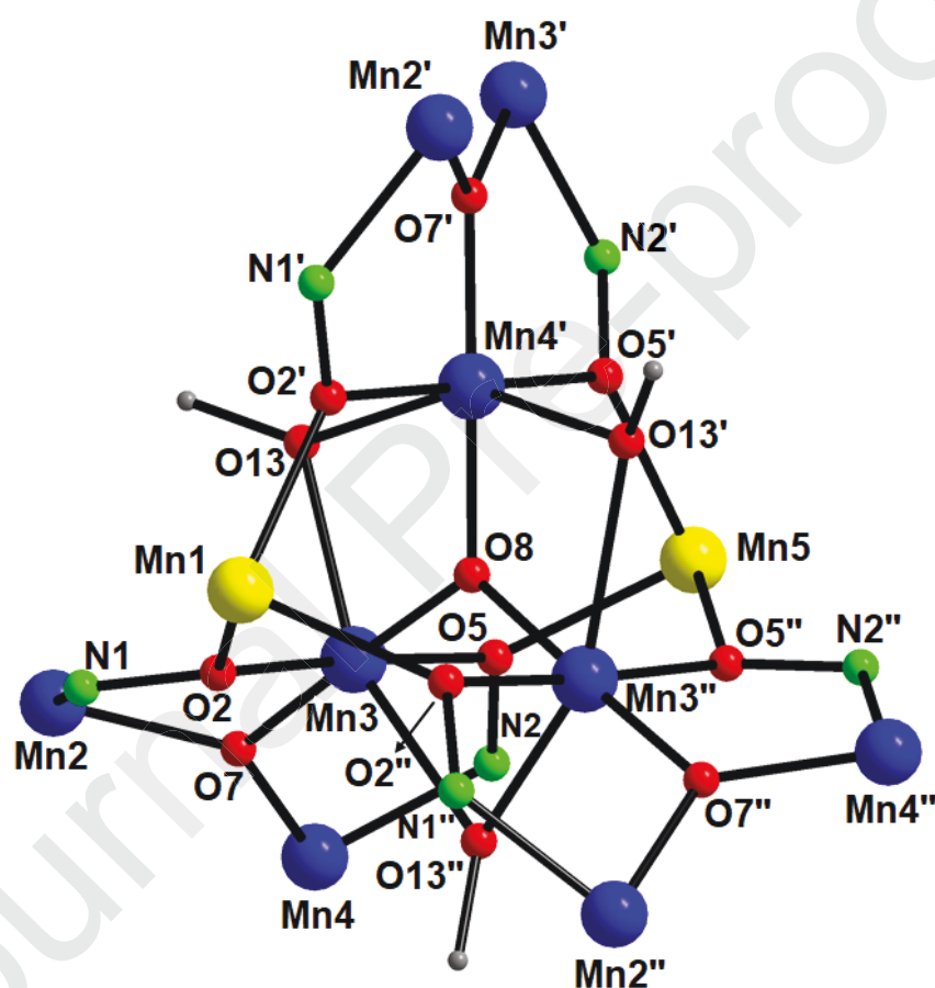
Fig. 3. Labeled representation of the complete [\text{Mn}^{\text{II}}_2\text{Mn}^{\text{III}}_9(\mu_3\text{-O})_4(\mu\text{-OR})_3(\mu_3\text{-NO})_6]^{14+} core of 1 . Color scheme and symmetry codes as in Fig. 1.
