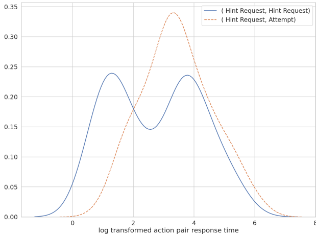
Figure 3: distribution curve of (Hint Request, Attempt) and (Hint Request, Hint Request) action pairs, when their first action was asking for hint after reading the problem, using natural log-transformed values of time taken for each action pair
