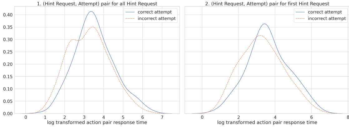
Figure 6: The amount of time a user spends after getting a hint is the same for students who made a correct or an incorrect attempt
