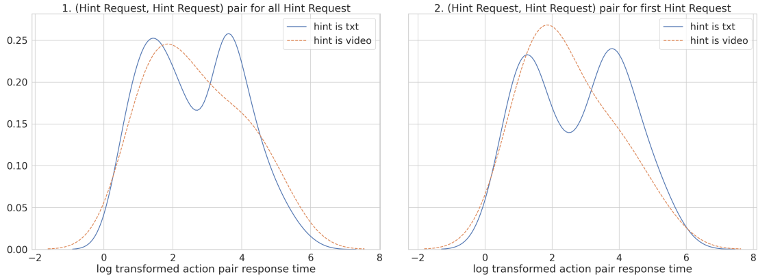
Figure 4: There are too few instances of video hint for us to draw a conclusion but the data does seem to indicate that the type of hint does not influence the action pair response time
