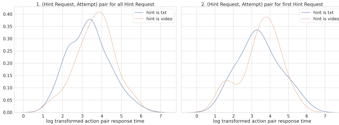
Figure 5: There are too few instances of video hint for us to draw a conclusion but the data does seem to indicate that the type of hint does not influence the action pair response time
