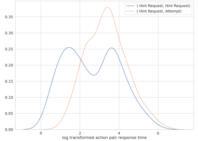
Figure 2: distribution curve of (Hint Request, Attempt) and (Hint Request, Hint Request) action pairs using natural log-transformed values of time taken for each action pair
