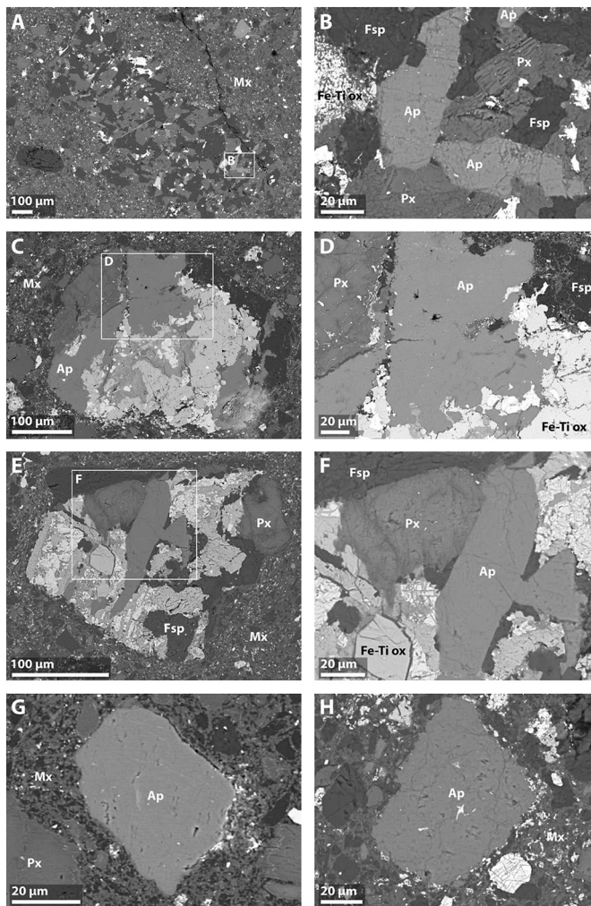
Fig. 1. Backscattered electron images of NWA 7034 apatite in: (A, B) a basaltic clast, (C–F) FTP clasts, and (G, H) interclastic matrix. White boxes indicate the regions shown at higher magnification images in adjacent panels. Ap = apatite, Fsp = feldspar, Fe-Ti ox = Fe-Ti oxide, Mx = matrix, Px = pyroxene.
