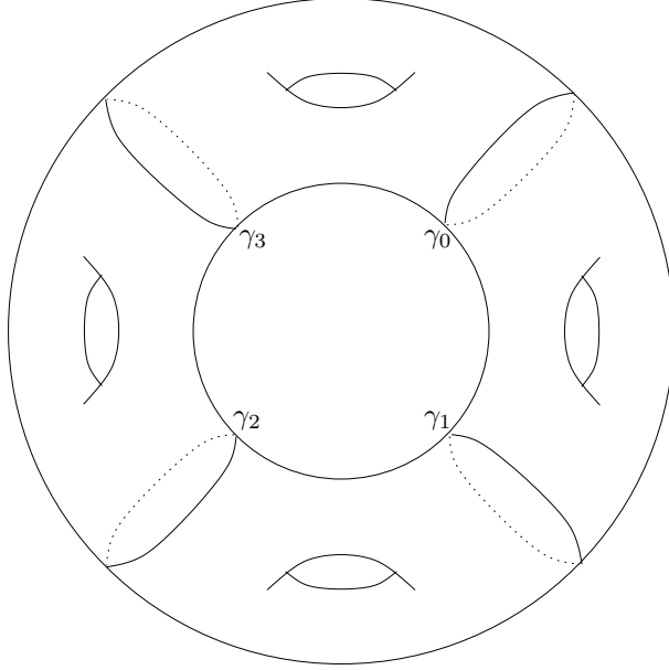
FIGURE 3. The pairwise disjoint curves \gamma_0, \dots, \gamma_{m-1} for the second family in the case of genus 5 (and hence m = 4 ).
