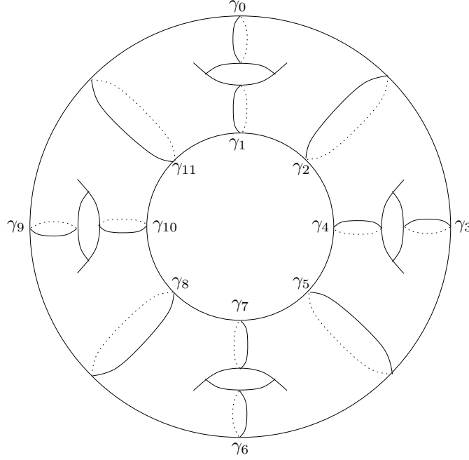
FIGURE 2. The pairwise disjoint curves \gamma_0, \dots, \gamma_{m-1} for the first family of examples in the case of genus 5 (and hence m = 12 ).
