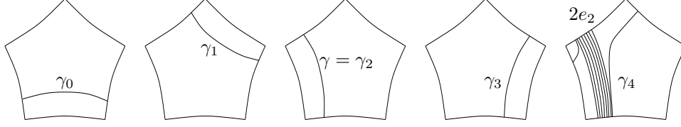
FIGURE 1. The curves \gamma_0, \dots, \gamma_4 in S_{0,4} . Any five consecutive curves \gamma_{k-2}, \dots, \gamma_{k+2} differ from those shown here by a homeomorphism, and replacing e_2 by e_k .
