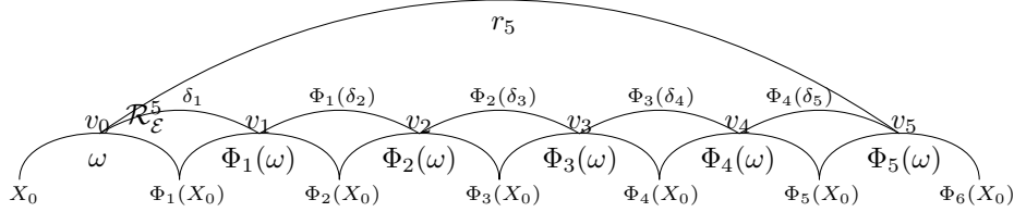
FIGURE 3. The concatenation of geodesic segments \delta_1, \Phi_1(\delta_2), \dots, \Phi_4(\delta_5) defining R_{\mathcal{E}}^5 \subset R_{\mathcal{E}} and \omega \cup \Phi_1(\omega) \cup \dots \cup \Phi_5(\omega) \subset g_{\mathcal{E}}^{\omega} , together with the geodesic segment r_5 connecting the endpoints of R_{\mathcal{E}}^5 .
