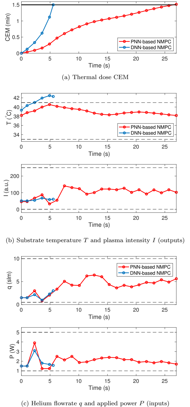
Fig. 6. Real-time control experiments. Experiments were repeated three times to ensure reproducibility of results in the face of the intrinsic stochasticity of plasma dynamics. Average profiles are shown here.
