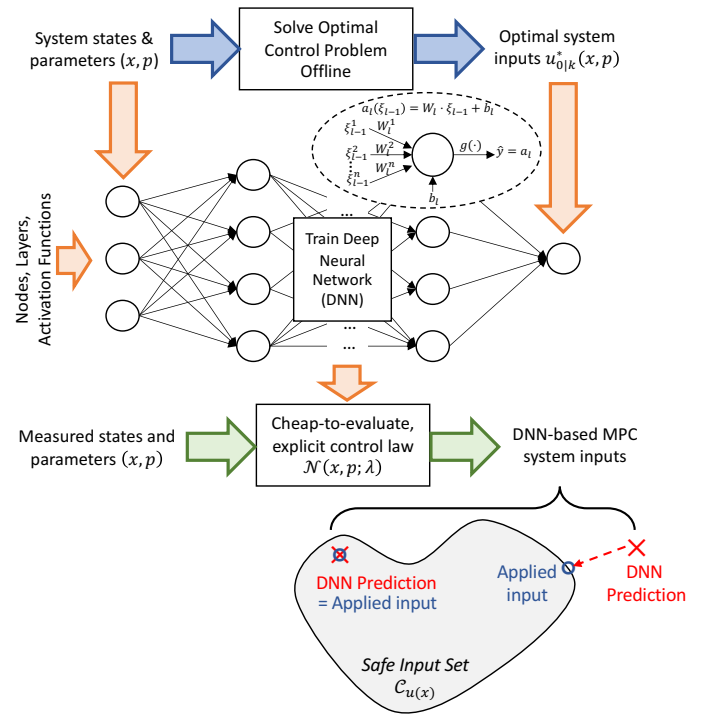
Fig. 2. The proposed fast approximate NMPC strategy with guaranteed closed-loop constraint satisfaction.
