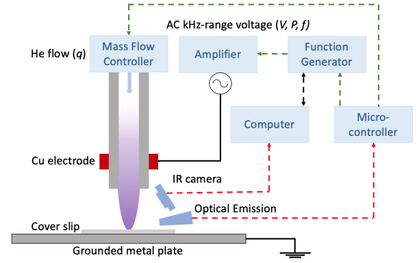
Fig. 1. Schematic of the APPJ testbed. The red dashed lines indicate measured outputs, whereas the green dashed lines indicate manipulated inputs.
