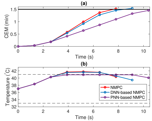
Fig. 4. Closed-loop simulation profiles of (a) CEM dose metric and (b) substrate temperature. The black solid line is the CEM setpoint while the dashed lines are the temperature constraints.
