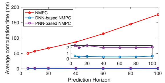
Fig. 5. Average online computation time of the NMPC, DNN-based NMPC, and PNN-based NMPC per iteration as a function of the prediction horizon.
