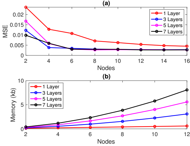
Fig. 3. (a) Mean squared error (MSE) and (b) memory footprint of the DNN approximation of the NMPC law as a function of number of nodes and layers.
