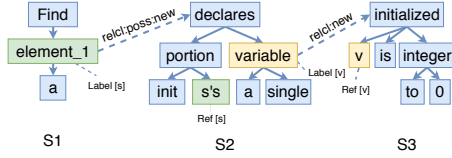
Figure 4. An illustration of dependency tree combination.
