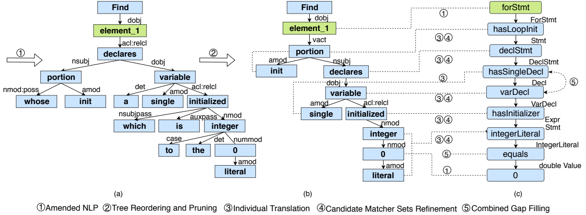
Figure 3. The synthesis process.
