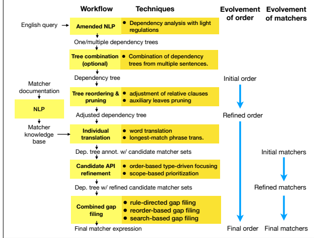
Figure 2. Overall workflow of Deepspy, its main techniques, and the enabled evolvement of the order and matchers of ASTMatcher expressions.
