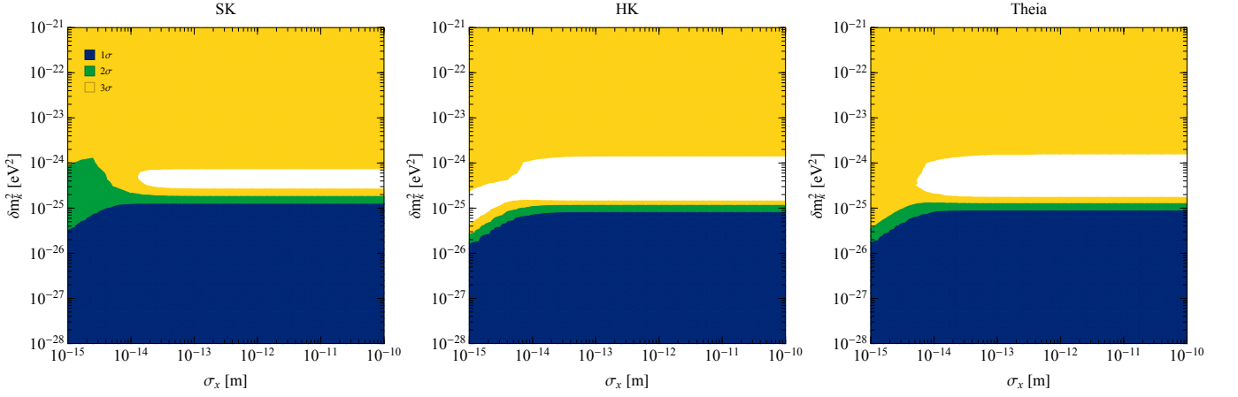
FIG. 10: Sensitivity on the (\sigma_x, \delta m_k^2) parameter space from ten years of simulated data at SK (left), HK (middle), and Theia (right). The regions that can be tested at less than or equal to 1\sigma, 2\sigma, 3\sigma level correspond to the blue, green and yellow areas, respectively. The white regions have a sensitivity > 3\sigma C.L.
