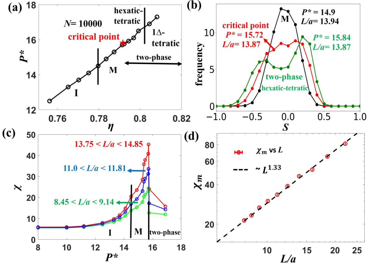
FIG. 3 (color online). Critical behavior of the equimolar disks+squares mixture with \xi = 1.1 and N = 10000 . (a) Equation of state, P^* vs. \eta ; the star marks the critical point at P^* = 15.72 and \eta = 0.791 and the vertical solid lines mark approximate boundaries between the I phase-M region and (hexatic-tetratic)-(1 \Delta -tetratic) two-phase regions. (b) Distribution of the local order parameter, S
