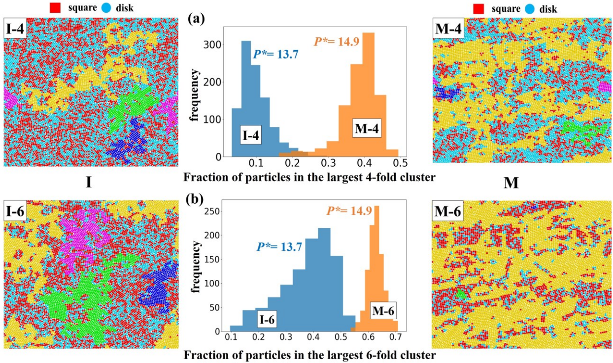
Fig. 7 (color online). Growth of the four-fold and six-fold ordered domains for the equimolar disks+squares mixture with \xi = 1.1 and N = 10000 for I phase (at P^* = 13.7 ) and the M region (at P^* = 14.9 ). Distribution function of the fraction of particles belonging to the largest four-fold (a) and six-fold (b) clusters. Representative snapshots for the I and M configurations are labelled as I-4 and M-4 for four-fold clusters and I-6 and M-6 for six-fold clusters. The particles belonging to the first, second, third, and fourth largest clusters are colored in yellow, green, magenta and blue, respectively.
