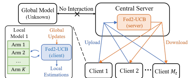
Figure 3: The FMAB framework.
