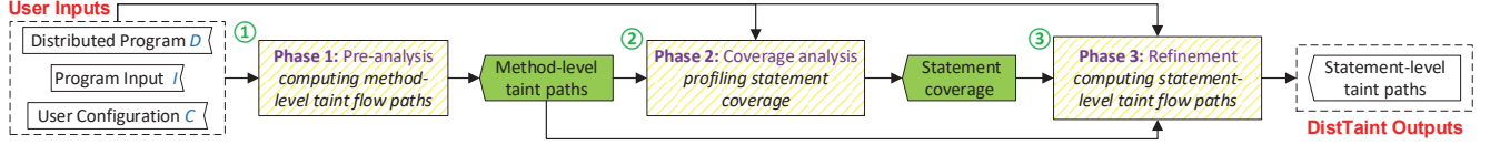
Figure 1: The overall workflow of the proposed technique for dynamic taint analysis of enterprise-scale distributed software.
