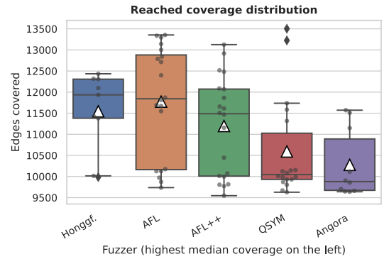
Figure 3: Example top five rankings for sqliteB.
