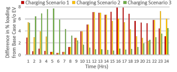
Fig. 6: Impacts on most heavily loaded transformer
