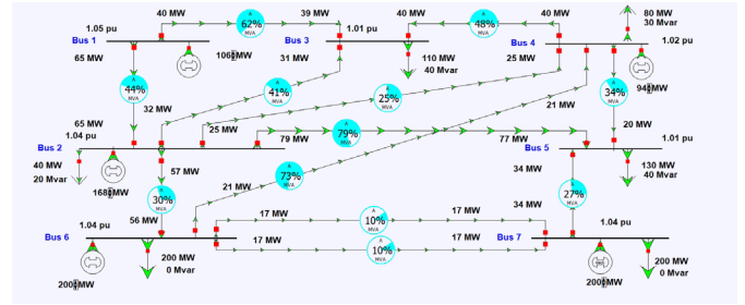
Figure 1: Seven Bus System Oneline
