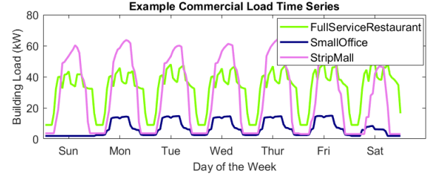
Fig. 3. Prototypical commercial building load time series examples by type
