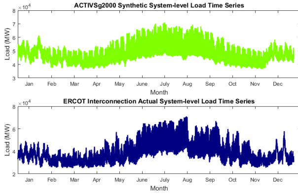
Fig. 9. ACTIVSg2000 synthetic system load V.S. ERCOT Interconnection system Load
