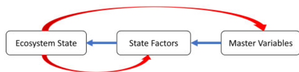
Figure 1: The traditional state factor model (blue arrows) including feedbacks (red arrows).
