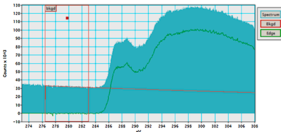
Fig. 3. Carbon electron energy loss spectrometry of yak dung biochar pyrolysed at 500 °C with a holding time of 2 h.
