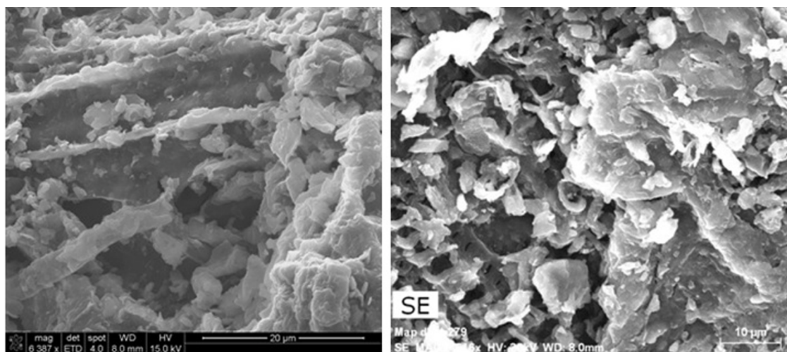
Fig. 2. Scanning electron microscope (SEM) image of yak dung biochar pyrolysed at 500 °C.
