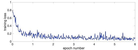
Figure 10: The cross entropy loss for the first six epochs of training the final layer of our vision-based model. (We adapted the Resnet18 CNN, pretrained on Imagenet). We can see that the model converges quickly.
