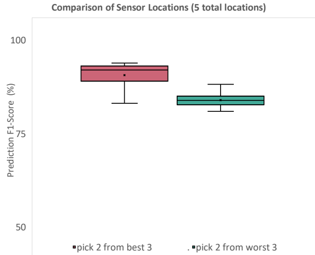
Figure 14: A box plot of the lying accuracy with two sensors chosen out of three, first in our most effective locations and second in less effective locations (as there are only 5 locations one is in both). This simulates random failure of a single sensor. Having more sensors than necessary adds redundancy to the system.
