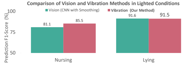
Figure 9: Results of Vision-based vs Vibration-based pig activity detection. Our Vibration-based method matches or slightly outperforms the Vision-based method in similar conditions.
