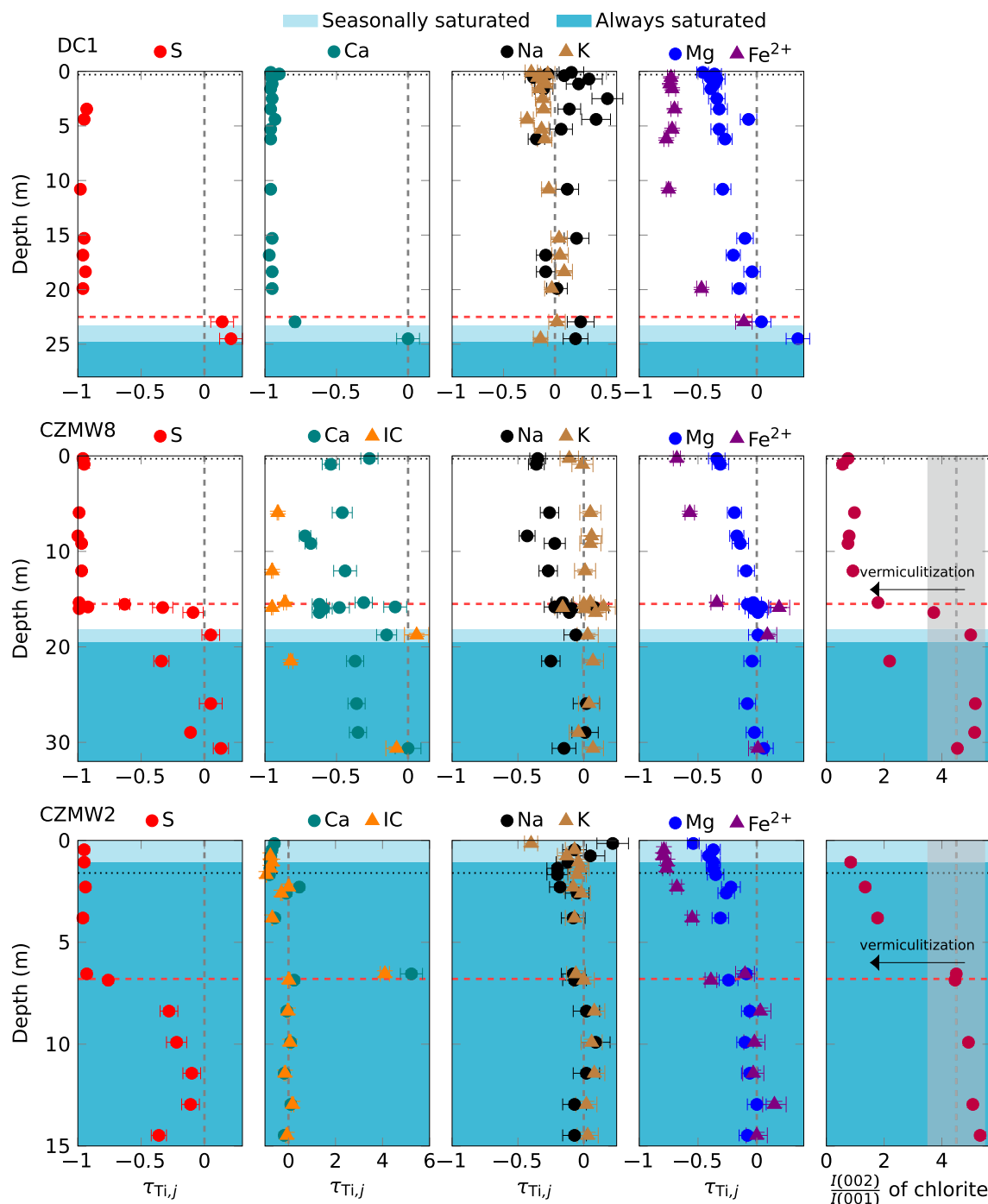
Fig. 4. Geochemical profiles at SSHCZO. The first four columns of panels are plots of \tau for S, inorganic carbon (IC), Ca, Na, K, Mg and ferrous iron ( \text{Fe}^{2+} ) in non-sulfide minerals, calculated assuming Ti as the immobile element in boreholes DC1, CZMW2 and CZMW8 (see Fig. 1b for the locations of these boreholes). The elemental measurements of samples from DC1, CZMW2 and CZMW8 were reported in Jin et al. (2010), Brantley et al. (2013) and Sullivan et al. (2016), respectively. The IC concentrations for CZMW8 are reported in Table S1. The IC concentrations for CZMW2 were calculated as the difference between total carbon concentration (reported in Brantley et al., 2013) and a constant organic carbon concentration (0.1 wt.%, Table S1). The Ca and IC concentrations of the parent were determined as an average over all concentrations in protolith in each borehole (see text). Other elements of the parent were averaged over the concentrations in protolith from all boreholes (see Appendix B). The horizontal dashed red line depicts the pyrite depletion front, which separates the protolith and regolith (see text). The horizontal dashed black line depicts the interface between mobile soil and weathered rock. The last column shows the degree of vermiculitization by normalizing the X-ray diffraction peak intensity of chlorite 002 reflection ( \sim 7.1 \text{ \AA} ) to the peak intensity of chlorite 001 reflection (14.1–14.3 \text{\AA} ) on random powder mounts: the lower the ratio, the higher the degree of vermiculitization. The dashed vertical line represents the mean value for the parent (see data in Table 2), and the gray area shows two standard deviations. Not enough samples from the DC1 core were available to analyze IC nor the degree of vermiculitization.
