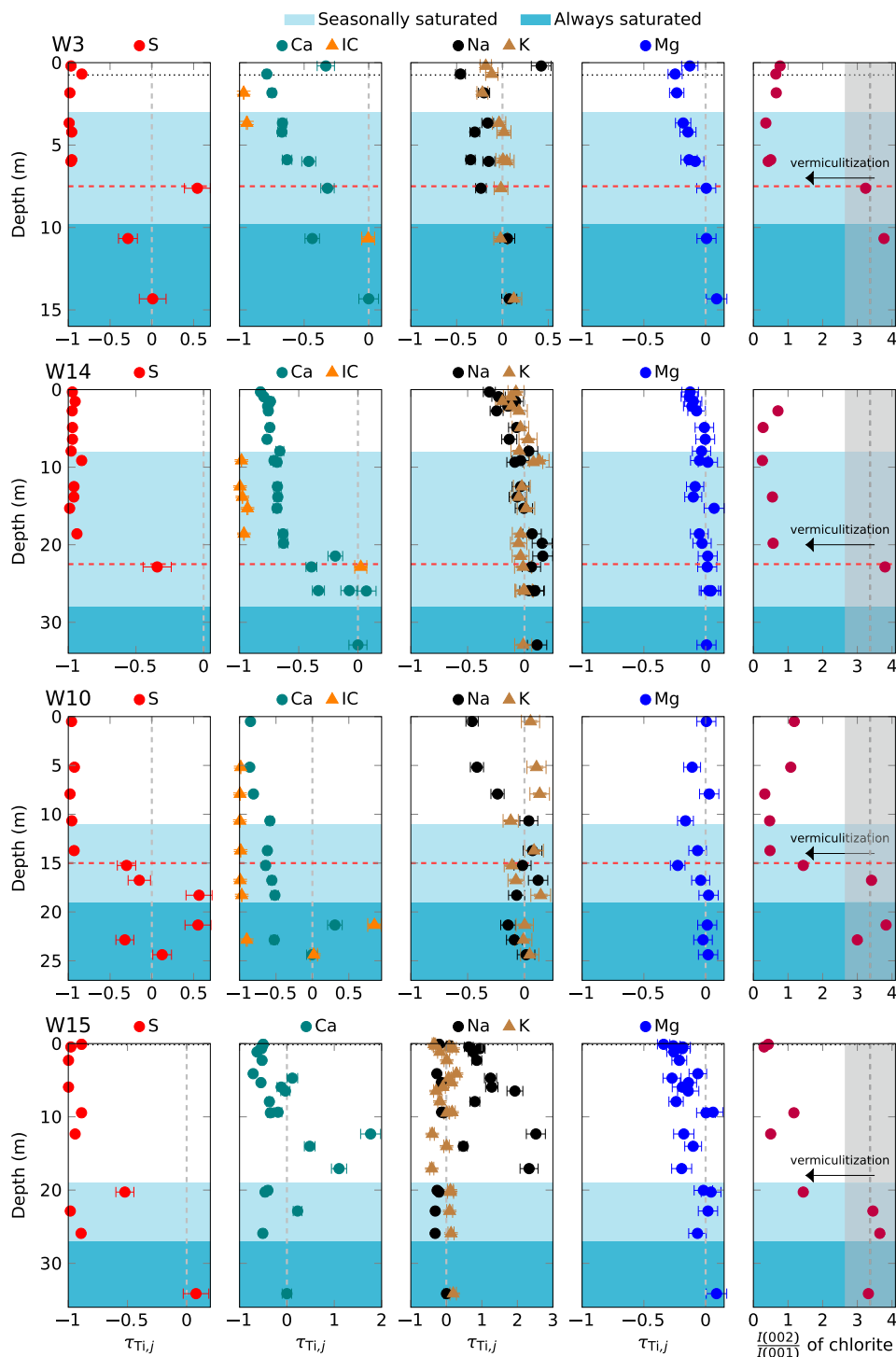
Fig. 5. Geochemical profiles at ERCZO. The first four columns of panels are plots of \tau for S, inorganic carbon (IC), Ca, Na, K, and Mg, calculated assuming Ti as the immobile element in boreholes W3, W14, W10, and W15 (see Fig. 1c for the locations of these boreholes). The elemental data are reported in Table 3. The parent concentrations were the average of the protolith from all the boreholes (see Appendix B). The dashed vertical line in the last column represents the mean value for the parent (see data in Table 2), and the gray area shows two standard deviations. The variation of concentrations of Na and Ca in borehole W15 indicates several zones in W15 are enriched in plagioclase but depleted in clay minerals and Ti. The description of the labels can be found in the caption of Fig. 4.
