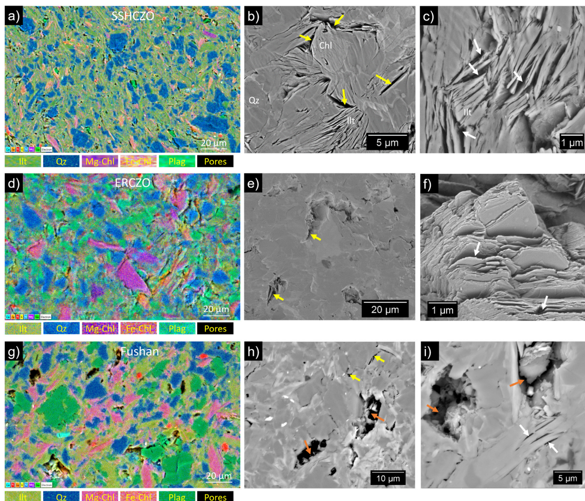
Fig. 2. X-ray elemental maps (a, d, g) and BSE images (b, c, e, f, h, i) of argon-ion-milled sections of unweathered shale from SSHCZO (borehole CZMW8, 23.8 mbfs, the top panels a-c), ERCZO (ERCZO_W10-75, 22.9 mbfs, the middle panels d-f) and Fushan (Fushan_FSC1_2, 14.8 mbfs, the bottom panels g-i). Images display the mineral fabric (spatial distribution and orientation) and pore morphology. The elemental map reflects a mixed backscattered electron and energy-dispersive spectroscopy signal. The small pores (<10 nm) observable under SEM are mainly intercrystalline or intracrystalline within phyllosilicates (white arrows). Larger pores are commonly observed along the boundary between silt-sized grains (yellow arrows). Dissolution features are observed in shale from Fushan (brown arrows). Color legend in left corner of elemental panels reports the dominant element. These data were then interpreted to indicate dominant minerals as shown: Illt: illite, Qz: quartz, Mg-Chl: Mg-rich chlorite, Fe-Chl: Fe-rich chlorite, Plag: plagioclase.
