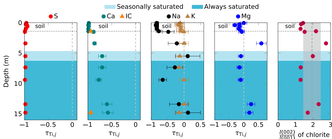
Fig. 6. Geochemical profiles of rock chips from Fushan. The first four columns of panels are plots of \tau for S, inorganic carbon (IC), Ca, Na, K, and Mg, calculated assuming Ti as the immobile element. The samples below soil-saprock interface were collected from borehole FSC1 near the valley and other samples were rock chips collected from a soil pit (FS1) nearby (see Fig. 1d for the locations). Sample FSC1_6 from 11.5 mbls and sample FSC1_13 from 4.4 mbls are from sandy interbeds and therefore are excluded in the plots. The elemental data are reported in Table 3. The parent concentrations were set equal to the average of the outcrop samples (see Appendix B). The dashed vertical line in the last column represents the mean value for the samples from the outcrop (see data in Table 2), and the gray area shows two standard deviations. The description on the labels can be found in the caption of Fig. 4.
