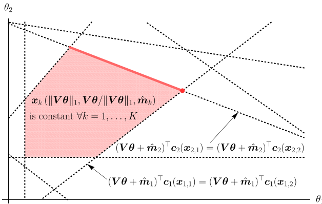
Figure 4. (Color online) Solution-Induced Hyperplane Arrangement
