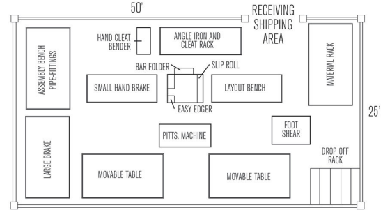
Fig. 7: Sheet metal shop floor layout [31]
