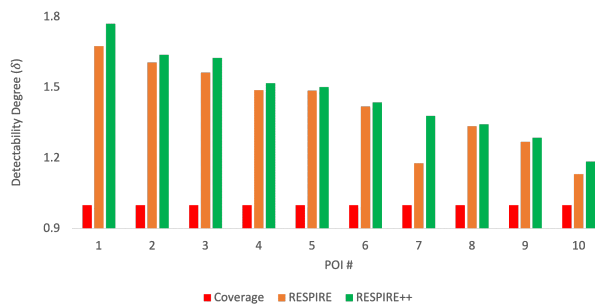
Fig. 8: Detectability degree comparison for sheet metal shop floor sensor placement
