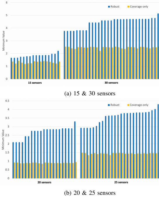
Fig. 4: Small room minimum detectability degree: Coverage [6], [7] vs. RESPIRE (a) 15-30 sensors (b) 20-25 sensors
