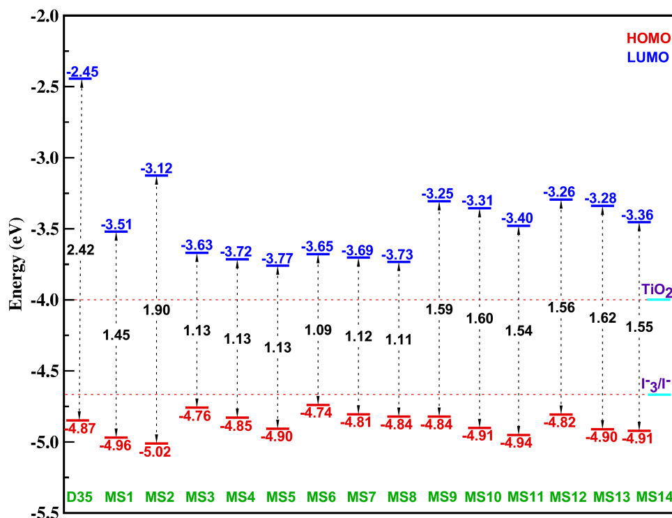
Fig. 5 Frontier molecular orbital (FMO) energies and energy gaps calculated at (U)B3LYP/6-31G(d, p) level of theory and basis set of the parent and designed dyes, compared with TiO 2 conduction band and I 3 - /I - oxidation potential.
