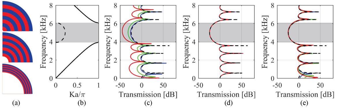
FIG. 2. (a) Quarter section of the EPC for r_0/a = 0.1 (top), r_0/a = 1 (middle), and r_0/a = 10 (bottom). Images do not have the same scale. (b) Dispersion relation for the EPCs [Eq. (7)] for a_1 = a_2 = 0.05m (dashed lines show imaginary Bloch wave number). Transmission curves for: (c) radially alternating homogeneous rings, (d) EPC1, and (e) EPC2, each plotted for r_0/a = 0.1 (red), r_0/a = 1 (green), r_0/a = 10 (blue), and compared to the equivalent Cartesian PC (black dashed).
