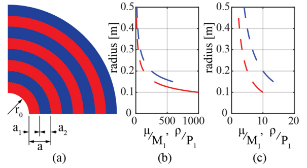
FIG. 1. (a) Quarter section of the effective phononic crystal for torsional wave propagation. (b) Radial dependence of material properties for EPC1 [Eqs. (4) and (5)]. (c) Radial dependence of material properties for EPC2 [Eqs. (8) and (9)]. The EPCs shown here have r_0/a = 1 .
