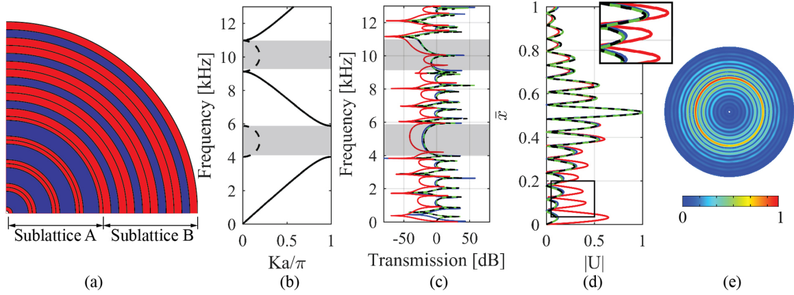
FIG. 3. (a) Quarter section of the superlattice for r_0/a = 0.1 . (b) Dispersion relation for the EPCs sublattices (dashed lines show imaginary Bloch wave number and shaded regions band gap frequencies). (c) Transmission from inner boundary to interface of the superlattice for homogeneous layers (red), EPC1 (green), EPC2 (blue), and equivalent Cartesian PC (black dashed). (d) Magnitude of modal displacement at interface mode frequency for homogeneous layers (red), EPC1 (green), EPC2 (blue), and equivalent Cartesian PC (black dashed) in terms of normalized spatial coordinate [ \bar{x} = (r - r_0)/(r_{\max} - r_0) for radial PCs and \bar{x} = x/x_{\max} for Cartesian PC]. The inset shows zoom-in view of modal displacements. (e) Normalized modal displacements of the EPC1 at the interface mode frequency.
