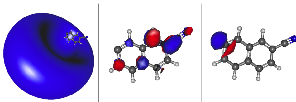
Figure 5. 2-cyanonaphthalene anion 7 a' HOMO (right); a'' valence state \pi LUMO (middle); and a' dipole bound state LUMO (left).
