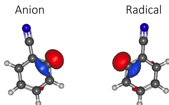
Figure 3. Benzonitrile anion geometry 2's a' HOMO (left) and the radical geometry 2's a' HOMO (right).
