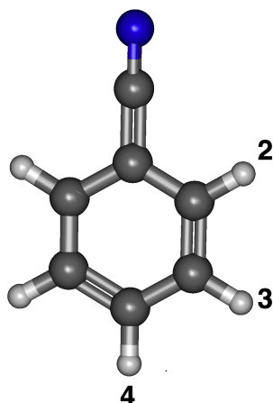
Figure 1. The optimized structure of benzonitrile with numbered positions of deprotonation.
