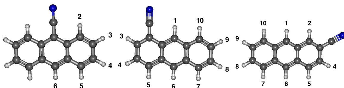
Figure 6. The optimized structure of cyanoanthracene derivatives with numbered positions for deprotonation.
