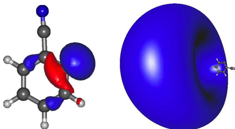
Figure 2. Benzonitrile anion 2 a' HOMO (left) and the a' LUMO (right) dipole bound orbital.
