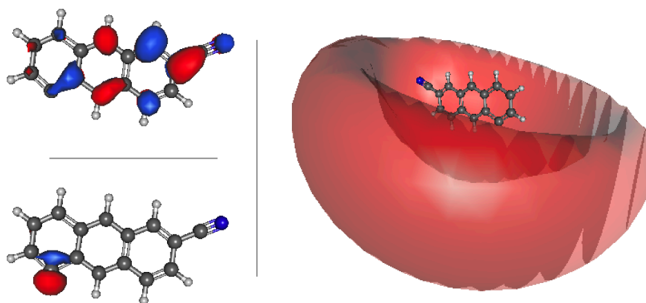
Figure 7. 3-cyanoanthracene anion 7 a' HOMO (bottom left); a'' valence state \pi LUMO (top left); and a' dipole bound state LUMO (right).
