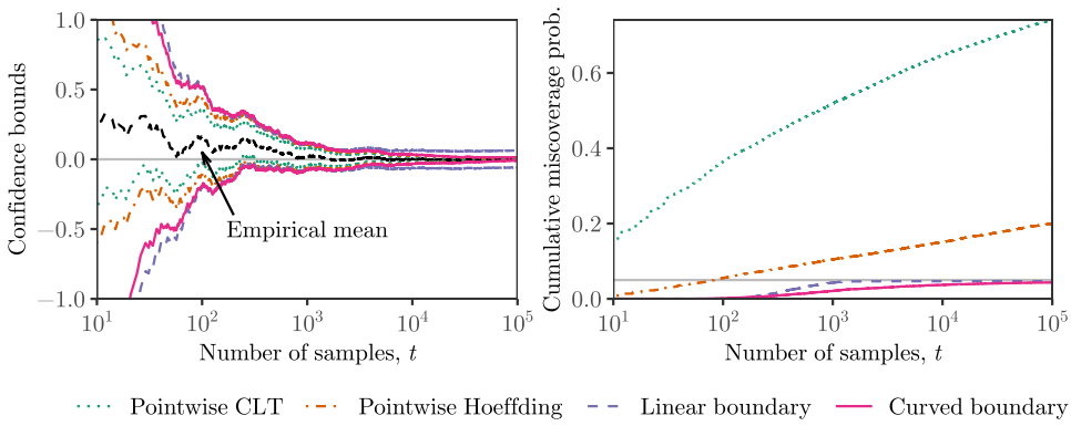
FIG. 1. Left panel shows 95% pointwise confidence intervals and uniform confidence sequences for the mean of a Rademacher random variable, using one simulation of 100,000 i.i.d. draws. Right panel shows cumulative chance of miscoverage based on 10,000 replications; flat grey line shows the nominal target level 0.05. The CLT intervals are asymptotically pointwise valid (these are similar to the exact binomial confidence intervals, which are nonasymptotically pointwise valid). The pointwise Hoeffding intervals are nonasymptotically pointwise valid. The confidence sequence based on a linear boundary, as in Lemma 1, is valid uniformly over time and nonasymptotically, but does not shrink to zero width. Finally, the confidence sequence based on a curved boundary is valid uniformly and nonasymptotically, while also shrinking towards zero width; here we use the two-sided normal mixture boundary, (3.7), qualitatively similar to the stitched bound (1.2).
