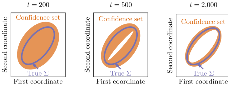
FIG. 6. The matrix confidence sequence of Corollary 5 based on one simulated sequence. Observations are drawn i.i.d. taking values \pm(\sqrt{2} \ \sqrt{2})^T, \pm(1/\sqrt{2} \ -1/\sqrt{2})^T each with probability 1/4 , with covariance matrix \Sigma = \frac{1}{4} \begin{pmatrix} 5 & 3 \\ 3 & 5 \end{pmatrix} , which is represented by the ellipse x^T \Sigma^{-1} x = 1 . Confidence ball with level \alpha = 0.05 is represented by shaded area between ellipses corresponding to elements of the confidence ball with minimal and maximal trace. Confidence sequence from Corollary 5 uses b = 4 and a discrete mixture boundary with \psi = \psi_G using c = 2b/3 , mixture density f_{1.4}^{\text{LIL}} from (A.51) with s = 1.4 matching (3.4), \eta = 1.1 and \bar{\lambda} = 0.262 chosen as described in Appendix E.
