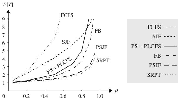
Fig. 8 Mean response time, E[T] , as a function of load for the M/G/1 with various scheduling policies. The job size distribution is a Weibull with mean 1 and C^2 = 10 . This figure taken from [90, p. 524]. Here, SJF refers to (non-preemptive) Shortest Job First, while PSJF refers to Preemptive Shortest Job First. FB is the Foreground-Background policy. PS is Processor-Sharing and PLCS is Preemptive Last-Come-First-Served
