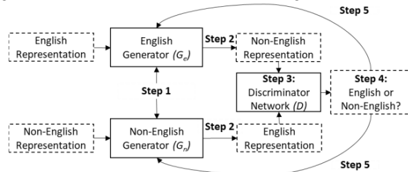
Fig. 5. Illustration of A-CLKT's Adversarial Learning Procedure
