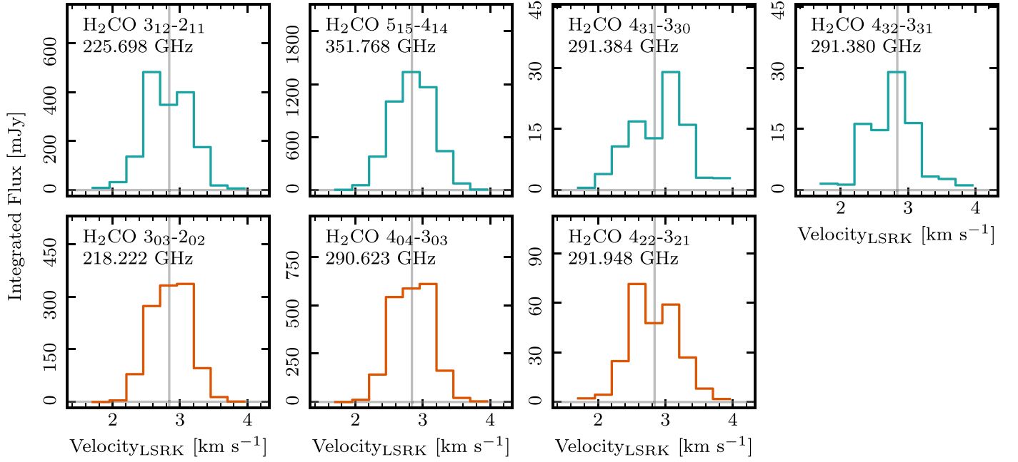
Figure 2. Integrated spectra of the seven observed Keplerian masked \text{H}_2\text{CO} transitions, i.e., pixels are masked according to a model predicting the Keplerian rotation of TW Hya. Top row, from left to right: o- \text{H}_2\text{CO} 3_{12}-2_{11} , 5_{15}-4_{14} , 4_{31}-3_{30} , and 4_{32}-3_{31} . Bottom row, from left to right: p- \text{H}_2\text{CO} 3_{03}-2_{02} , 4_{04}-3_{03} , and 4_{22}-3_{21} . The vertical line indicates the systematic velocity of TW Hya.
