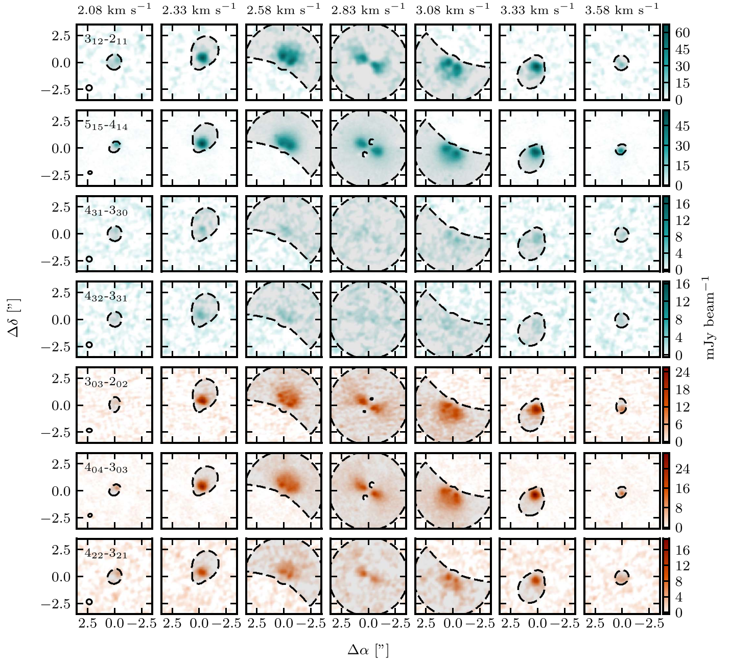
Figure 1. Channel maps from the observed transitions at native spatial resolution with the Keplerian masked overlayed. The channel velocities are labeled on top in the V_{\text{LSR}} reference frame. The teal and bronze color correspond to the ortho- and para-spin isomers, respectively. Beam sizes are indicated by the ellipse in the left-bottom corner of the first column.
