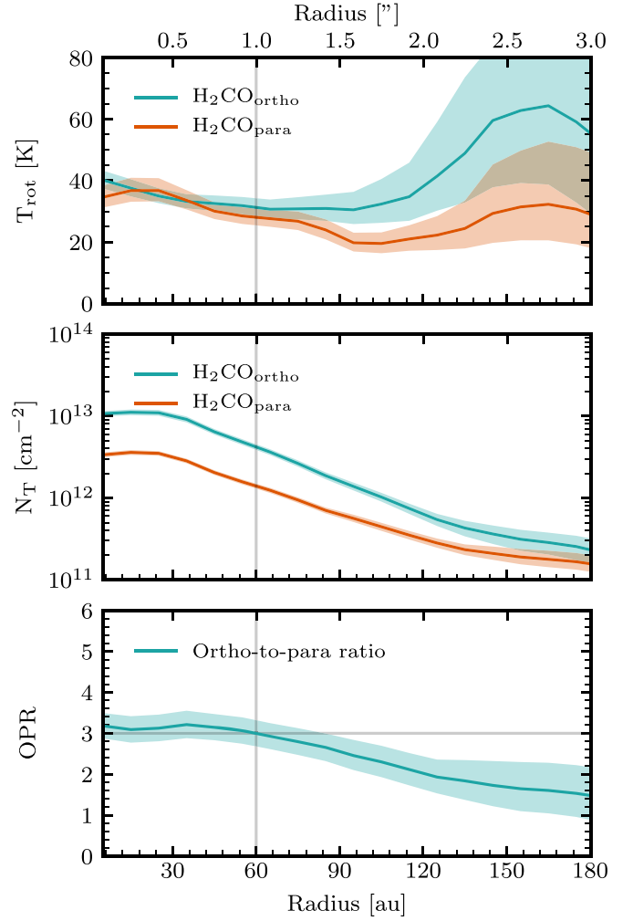
Figure 6. Radially resolved \text{H}_2\text{CO} temperature (top panel), column densities (middle panel), and OPR (bottom panel) of \text{H}_2\text{CO} obtained from our rotational diagram analysis using the radial emission profiles of Figure 4. The teal and bronze colors represent the ortho- and para-spin isomers, respectively. The shaded areas depict 1\sigma uncertainties. The gray vertical and horizontal lines depict the millimeter-dust continuum edge and the high temperature OPR limit of 3.0, respectively.
