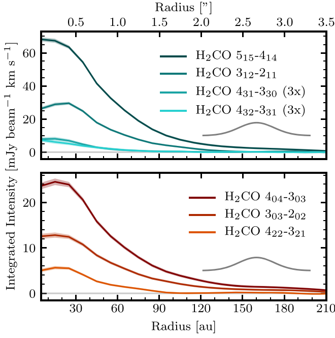
Figure 4. Radial intensity profiles of the observed ortho (top panel) and para (bottom panel) \text{H}_2\text{CO} transitions retrieved from the Keplerian masked moment-zero maps. The displayed uncertainties do not contain the 10% flux calibration error. All data have a common spatial resolution of 30 au depicted by the Gaussian in the bottom right.
