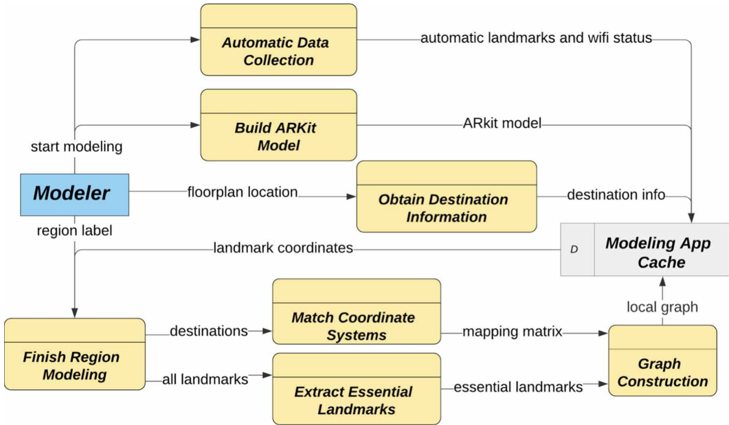
Figure 4. Local region modeling data flow diagram
