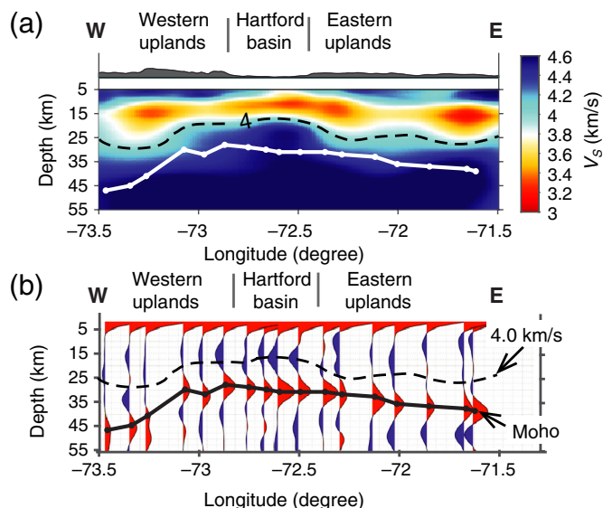
Figure 8. Initial results on crustal structure beneath northern Connecticut from the SEISConn project, after H. Gao et al. (unpublished manuscript, 2020; see Data and Resources ). (a) Shear-wave velocity profile along the SEISConn array, derived from full-waveform ambient-noise tomography. The dot-connected solid white line shows the estimated depth to Moho beneath each SEISConn station, from Long et al. (2019). Depths are estimated from the single-station migrated receiver function traces in (b). The dashed line shows the V_s = 4.0 km/s velocity contour, highlighting the high-velocity root, which is particularly prominent beneath the Hartford basin. (b) Single-station stacked radial-component receiver function traces, migrated to depth. Red pulses correspond to a positive velocity gradient (increase in velocity with depth), and blue pulses correspond to a negative velocity gradient (decrease in velocity with depth). Solid black line indicates estimated depths to the Moho across the profile, with the sharp step in crustal thickness visible in the western portion of the array. Dashed line indicates the V_s = 4.0 km/s velocity contour from the model shown in (a). E, east; W, west. The color version of this figure is available only in the electronic edition.
