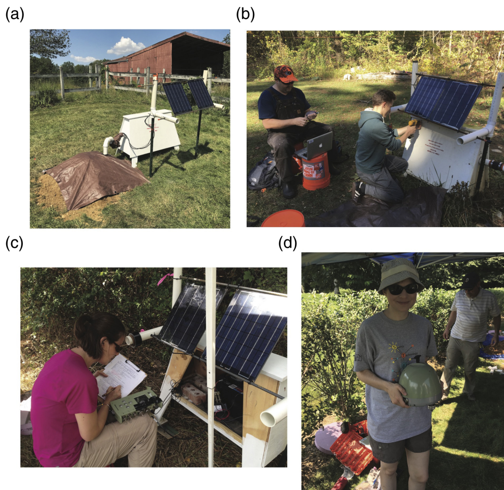
Figure 3. Field photos from the SEISConn seismic deployment. (a) Photo of a completed station (CS11 in Willington, Connecticut, installed in August 2017), showing the wooden electronics enclosure, the solar panel mount, and the buried vault (covered with dirt and tarp for thermal insulation). (b) Visit to station CS03 (Norfolk, Connecticut) for servicing in October 2017; photo shows removal of the front panel of the electronics enclosure. (c) Configuration of electronics system during installation of station CS14 (Thompson, Connecticut) in September 2015. (d) Preparing to install the sensor at station CS09 (Ellington, Connecticut) in August 2017. The color version of this figure is available only in the electronic edition.
