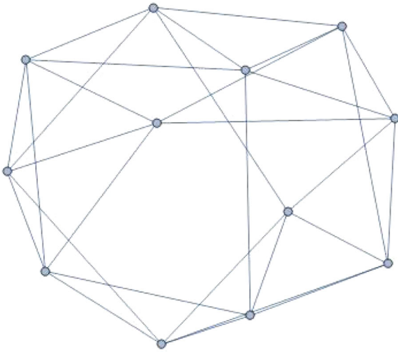
Figure 6. An asymmetric 5-regular Hamiltonian graph with 12 vertices.
