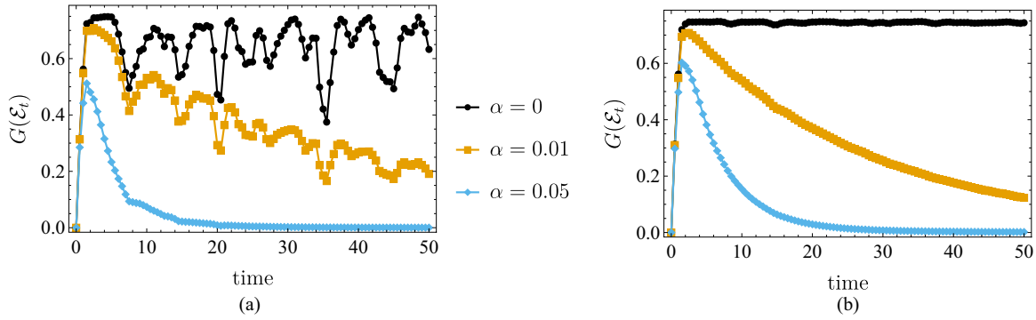
FIG. 2. Temporal variation of the open OTOC G(\mathcal{E}_t) for the TFIM Eq. (30) with L = 6 spins. The three curves correspond to varying choices of the dissipation strength \alpha in the Lindblad operators, Eq. (28). The chaotic ( g = -1.05, h = 0.5 ) and integrable ( g = 1, h = 0 ) phases are clearly distinguishable for the \alpha = 0 case (closed system); however, increasing the dissipation strength to \alpha = 0.05 makes them fairly indiscernible and destroys the revivals (or fluctuations) characteristic of integrable systems.
