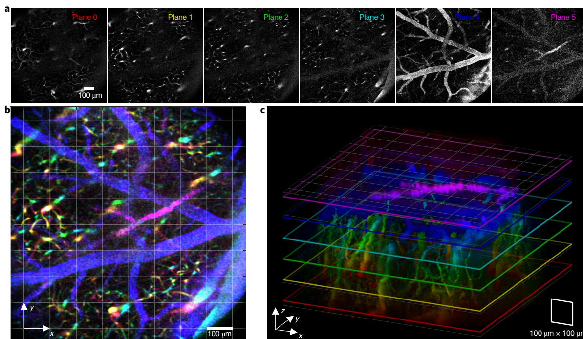
Fig. 2 | Reverberation 2PM imaging of in vivo mouse brain vasculature. a , Six independent reverberation planes at different depths from a single image with \Delta z of \sim 90\mu\text{m} . b , Merged image comprising the six planes; color indicates plane and depth (the single color of each plane merged in overlapping regions). c , Maximum intensity projection of z-stack (using short physical z-scan to fill in the gaps between reverberation planes) with slices from all six reverberation planes merged into a volume; color indicates depth. (Fly-through and fly-around are provided in Supplementary Videos 1 and 2.) Planes highlighted in c correspond to those in a and b . All images are corrected for crosstalk.
