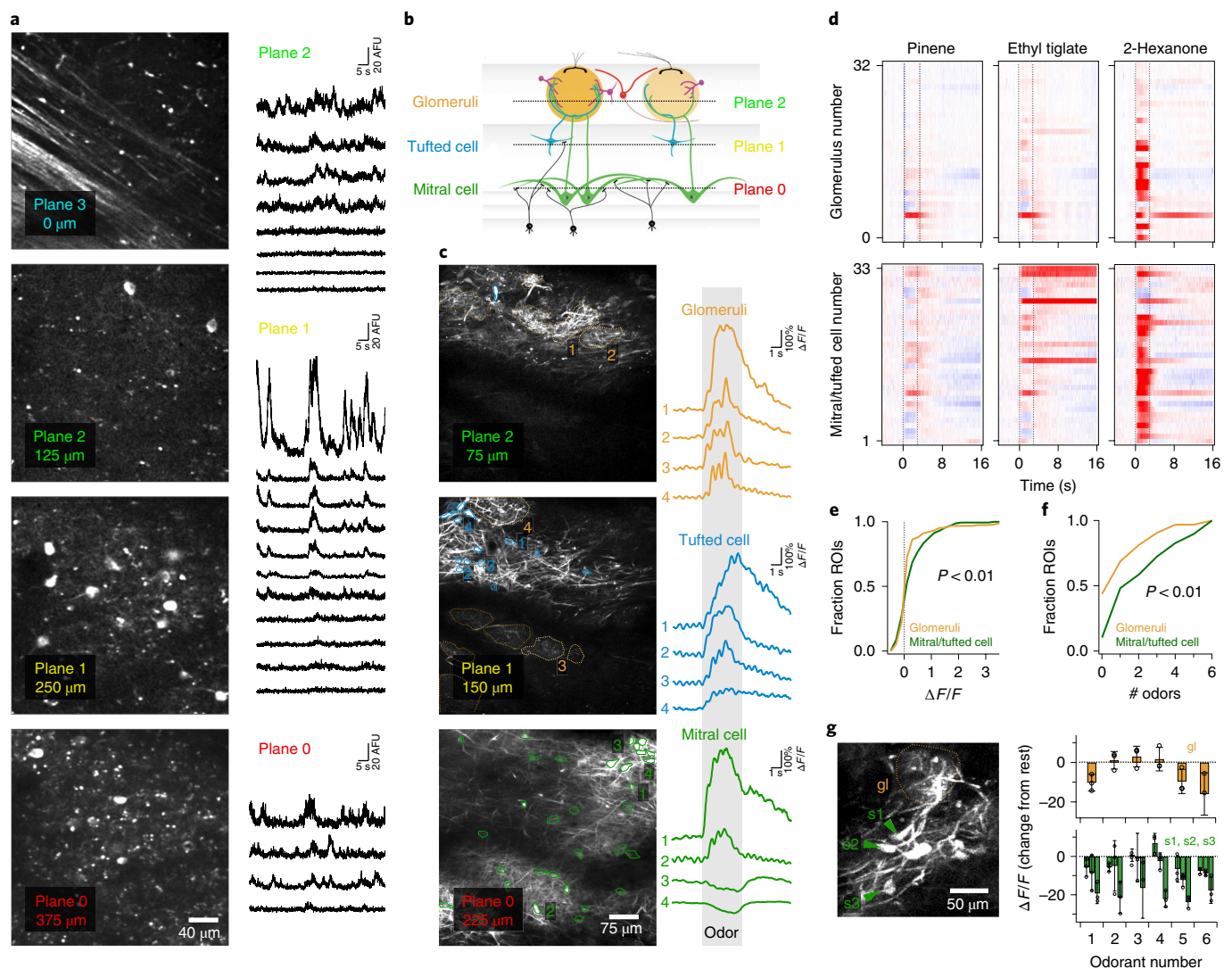
Fig. 3 | Reverberation imaging of in vivo mouse brain neural activity. a , Time-averaged x-y images of GCaMP6s-expressing neurons from four different planes of neocortex, with the top plane positioned at the brain surface (Supplementary Video 3). Traces to the right show the activity of individual neurons imaged in different sub-surface layers. b , Schematic showing the intersection of imaging planes with neuropil and cell types at different depths, modified from ref. 2 . c , Time-averaged x-y images of dendrites and somata of GCaMP6f-expressing neurons imaged in three different planes of main olfactory bulb (Supplementary Video 4). To the right, representative traces showing sensory responses to the odorant ethyl tiglate in postsynaptic dendrites (gold) and somata of two different classes of olfactory-bulb projection neurons (blue, green). d , Heat maps showing sensory responses in 32 glomeruli (top, containing postsynaptic dendrites) and 33 mitral/tufted somata (bottom) measured in a separate mouse (z-stack in Supplementary Video 5). Three representative odorants shown of six total. (Corresponding regions of interest (ROIs) are shown in the Supplementary Information.) e , Comparison of the distribution of response strengths for glomeruli (gold) and mitral/tufted cells (green). Mitral cells showed a significant shift towards stronger sensory responses ( P = 0.29 \times 10^{-3} , two-sided Kolmogorov–Smirnov test; n = 32 glomeruli, 33 mitral cell somata). f , Comparison of odorant selectivity for glomeruli and mitral cells. On average, mitral cells responded to significantly more odorants than glomeruli ( P = 6.5 \times 10^{-3} , two-sided Mann–Whitney test; n = 32 glomeruli, 33 mitral cell somata). g , Example of simultaneous imaging of postsynaptic dendrites (gold) and somata of three different mitral/tufted cells (green; s1, s2, s3) contained within a single glomerulus (gl). Bar plots show average response profiles across the panel of six odorants ( n = 3 trials, error bars represent \pm 1 s.d.). In this example, odor responses largely caused suppression relative to resting activity levels.
