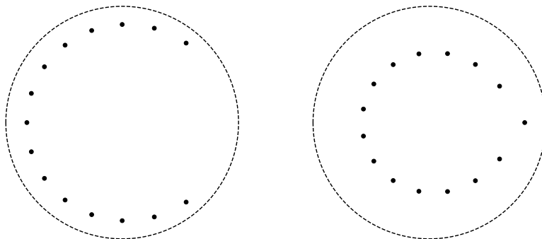
Fig. 1. Zeros of the extremal Blaschke products of Example 7.2.
