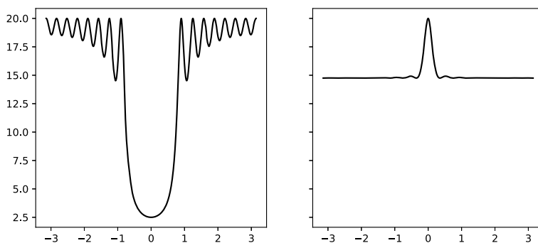
Fig. 2. Derivative of the extremal Blaschke products of Example 7.2.
