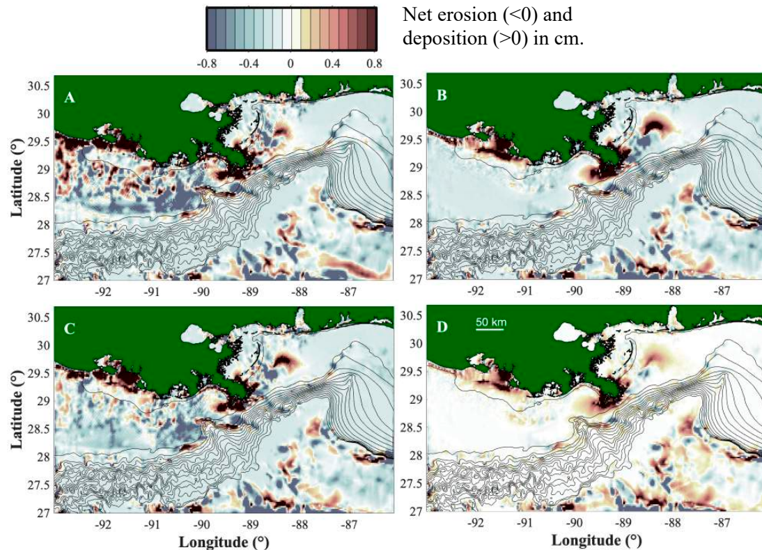
Figure 8. Net erosion (<0) and deposition (>0) calculated for suspended sediment transport for (A) entire model run (1 October 2007–20 September 2008); (B) prior to hurricanes: time-integrated from 1 October 2007 up until 25 August 2008; (C) during Hurricane Gustav; (D) during Hurricane Ike. Bathymetric contours (in black) drawn for depths of 10, and every 100 m up to 1500 m.
