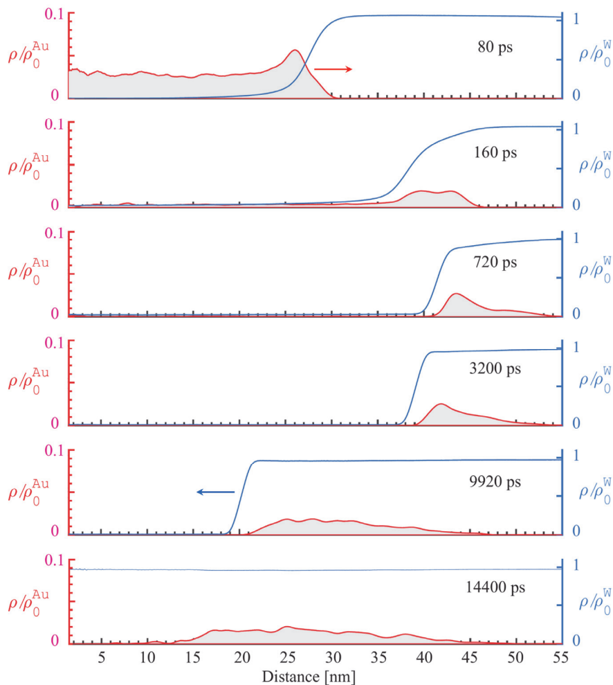
Figure 9. The water and Au density profiles plotted for different moments of time during the simulation illustrated by snapshots shown in Figure 6. The profiles are shown by blue lines for water and by red lines outlining grey areas for Au. The two arrows show the dominant processes driving the generation of the nanobubble (expansion of the products of the explosive decomposition of the nanoparticle, red arrow) and the collapse of the nanobubble (Laplace pressure produced by the surface tension, blue arrow). An animation showing the evolution of the density profiles is provided in Supporting Information for this article.
