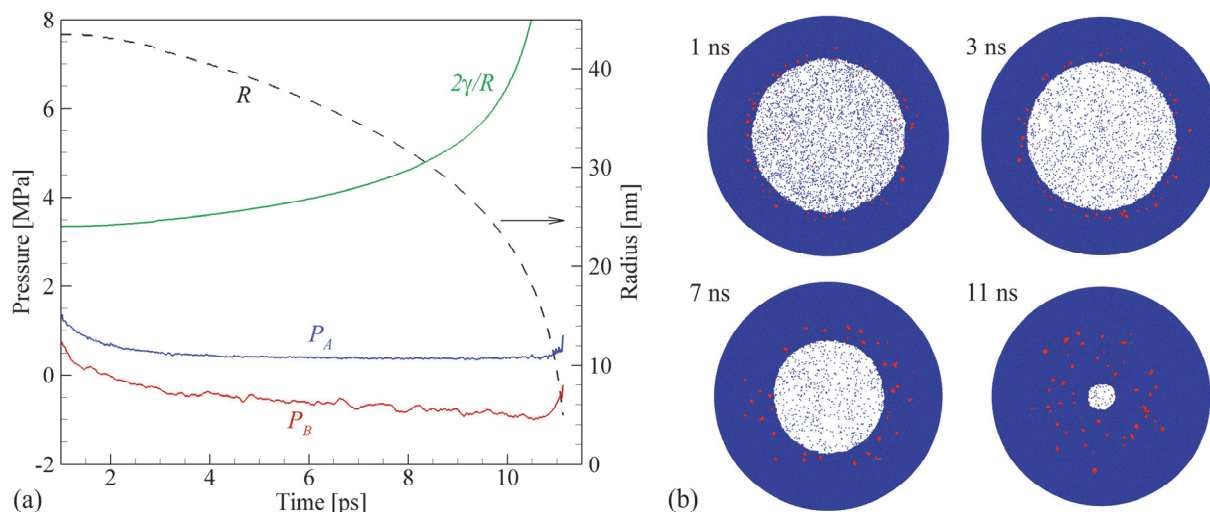
Figure 8. (a) The evolution of the radius of the nanobubble R , the corresponding Laplace pressure 2\gamma/R , the pressure inside the nanobubble P_A (averaged over region A in Figure 7b), and pressure P_B outside the nanobubble (averaged over region B in Figure 7b). (b) Snapshots of 4-nm-thick slices cut from the middle of the simulation system and shown for 1 ns, 3 ns, 7 ns, and 11 ns. The Au atoms and CG water particles in the snapshots are colored red and blue, respectively.
