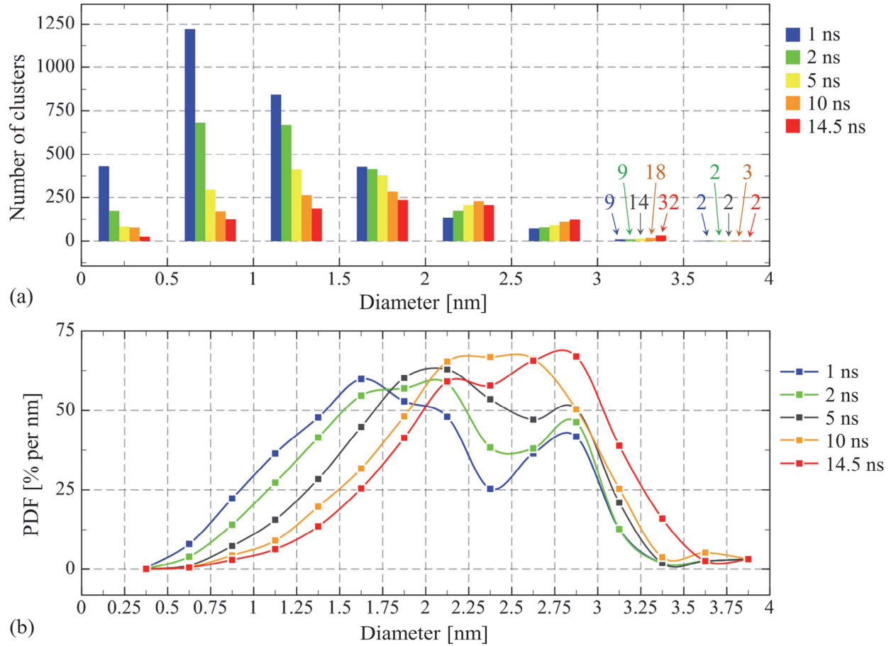
Figure 11. The evolution of the cluster/nanoparticle size distribution during the simulation of LFL illustrated in Figure 6, shown in the form of the number of clusters (a) and the probability density function of the cluster mass distribution (b). Clusters are separated by diameter into bins with
