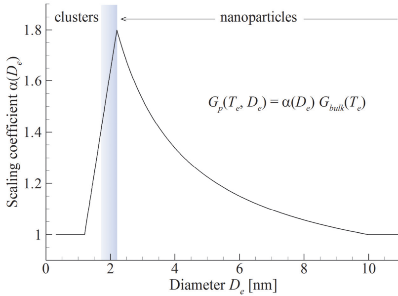
Figure 2. Scaling coefficient \alpha(D_e) used for an approximate representation of the dependence of the electron-phonon coupling factor on the Au nanoparticle diameter D_e . The shaded area marks the nanoparticle size range that corresponds to the transition between the metallic (plasmonic) and molecular (discrete/excitonic) type of the electronic structure.
