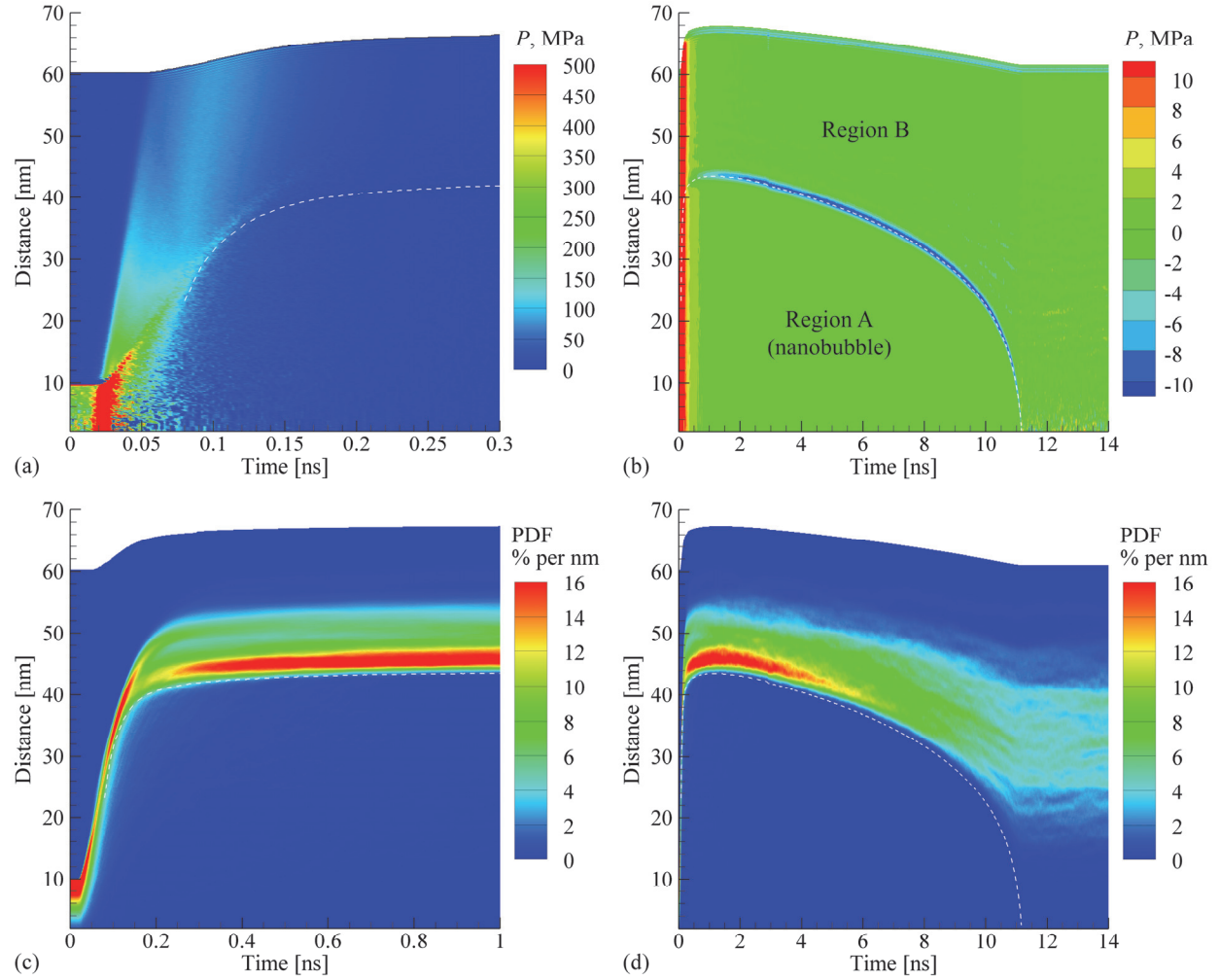
Figure 7. Spatial and temporal evolution of pressure (a, b), and probability density function (PDF) characterizing the distribution of Au atoms (c, d) predicted in the simulation for which snapshots are shown in Figure 6. The contour plots are shown for the initial stage of the fragmentation process (300 ps for pressure and 1 ns for PDF) in the left panels (a,c) and for 14 ns in the right panels (b,d). The white dashed lines mark the boundary of the emerging nanobubble, defined as a location where water density drops by 50% with respect to the initial value. The evolution of average pressure in Regions A and B marked in (b) is shown in Figure 8a.
