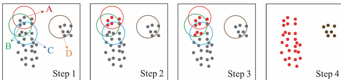
Figure 3. Schematic of a series of steps in the serial cluster analysis algorithm. Atoms without cluster ID are colored gray. Atoms assigned different cluster IDs are colored by different colors.
