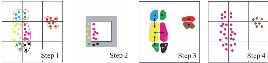
Figure 4. Schematic of the on-the-fly parallel cluster analysis algorithm. Each square represents a region treated by a single processor. Atoms are colored by the cluster IDs. The gray region in Step 2 is a skin layer where the atoms sent by neighboring processors are located. Colored areas in Step 3 show different parts of clusters joined together by the master processor. Arrows in Step 3 show the pairs of local clusters identified at Step 2.
