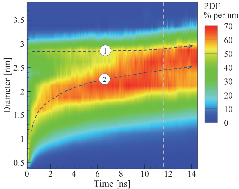
Figure 10. The evolution of the mass-weighted cluster/nanoparticle size distribution in a simulation of LFL illustrated in Figure 6. The distribution is shown in the form of the probability density function calculated by dividing the total mass of clusters/nanoparticles that fall within size bins with a width of 0.25 nm by the bin width and by the total mass of Au in the system, and then multiplying by 100 to express PDF in units of % per nm. The two gray dashed arrows show two
